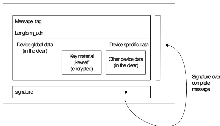
Figure 17: domain_registration_response() message
