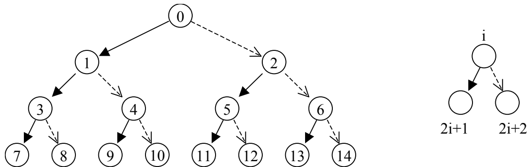
Figure 32 Subscriber group node (and node key) numbering
