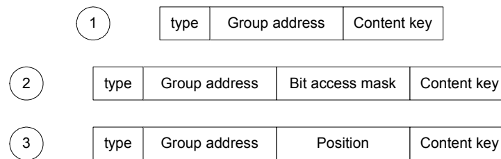
Figure 31: Addressing modes
