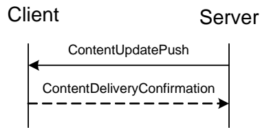
Figure 18: Content Update Push transaction
