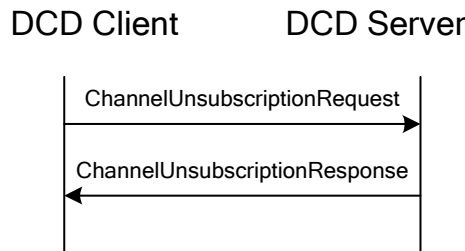
Figure 30: Channel Unsubscription message flow
