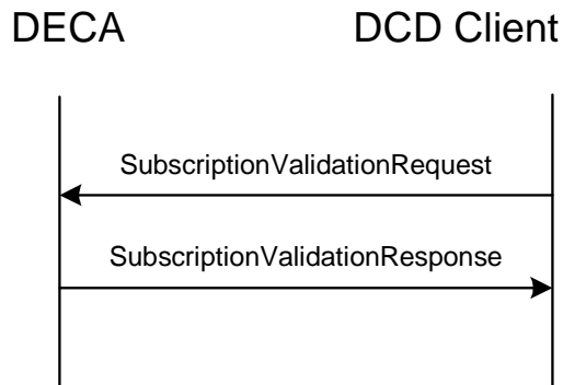
Figure 62: Subscription Validation transaction
