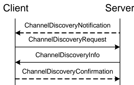
Figure 34: Channel Discovery Notification / Pull Transactions
