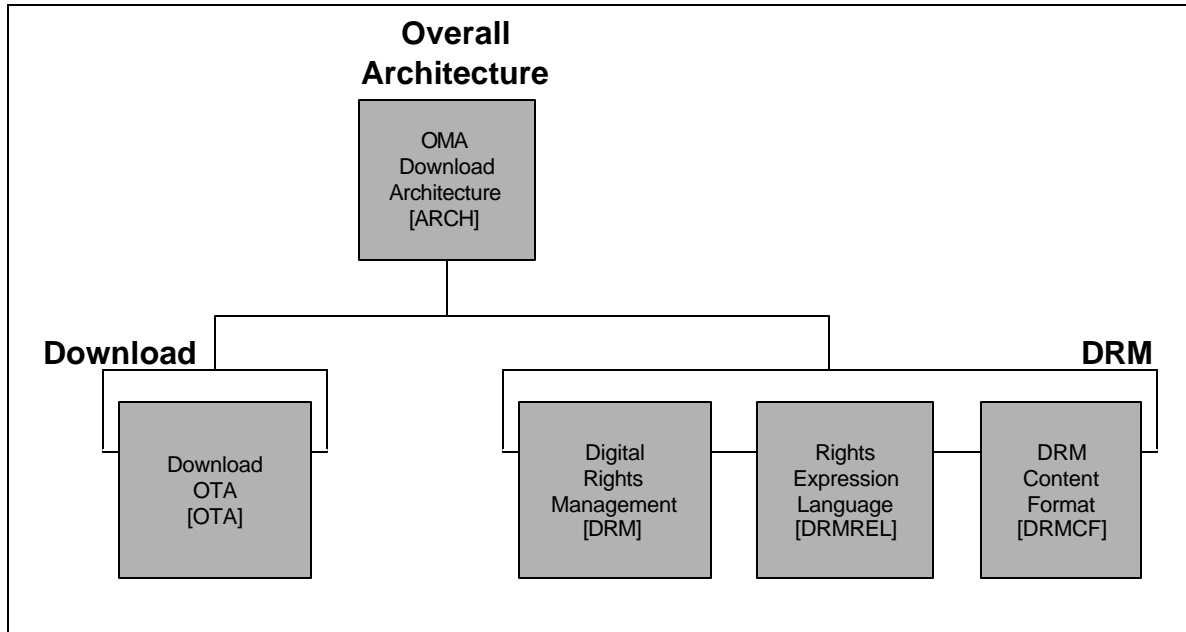
Figure 1 Documents Overview.
