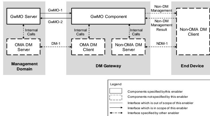
Figure 3: Adaptation Mode GwMO Architectural Diagram Using Interfaces
