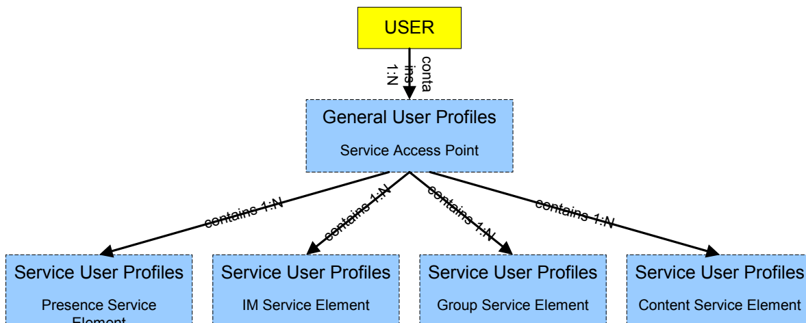
Figure 3: User Profiles
