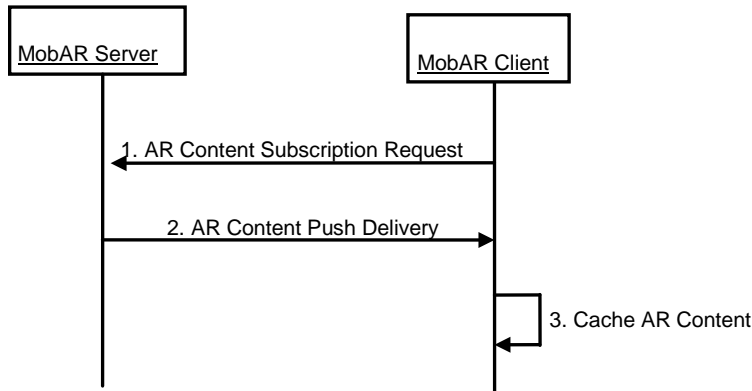
Figure 6: AR Content Push Delivery Call Flow
