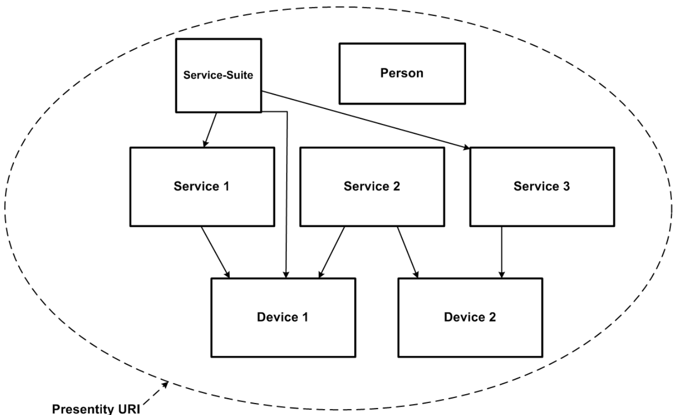
Figure 1: Relationship between components of the Presence Data Model
