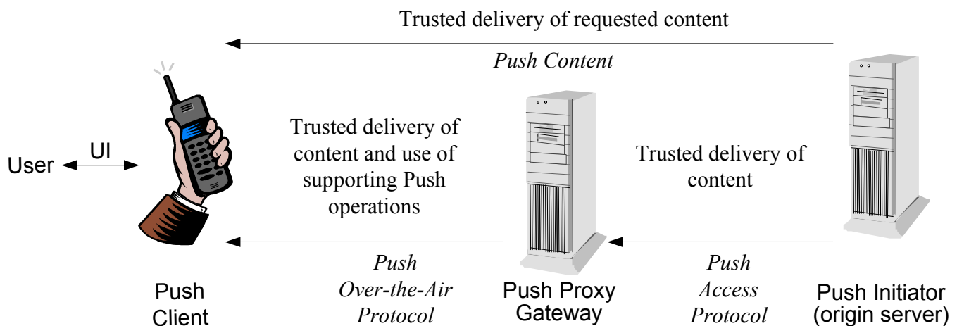
Figure 1: Push Framework
