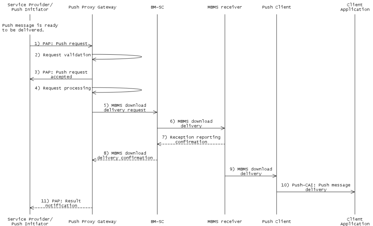
Figure 15: Push/MBMS Message Delivery example
