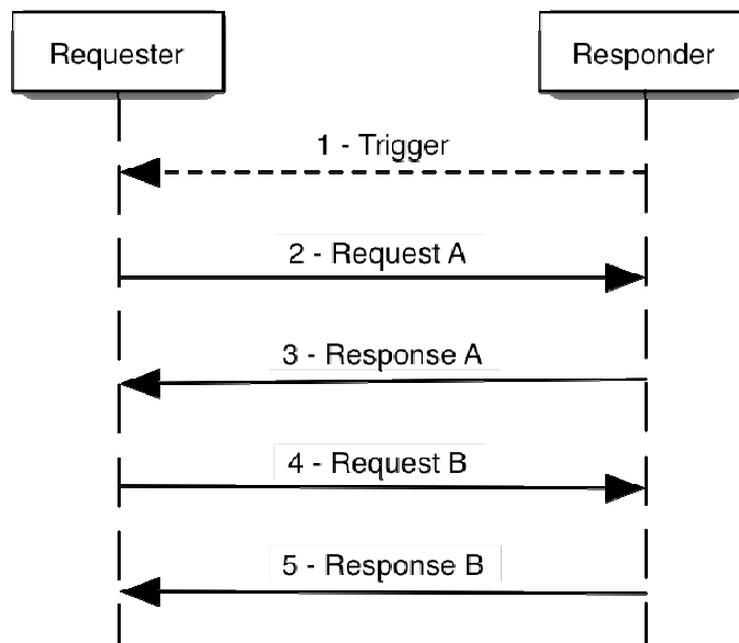
Figure 1 - Communications Model
