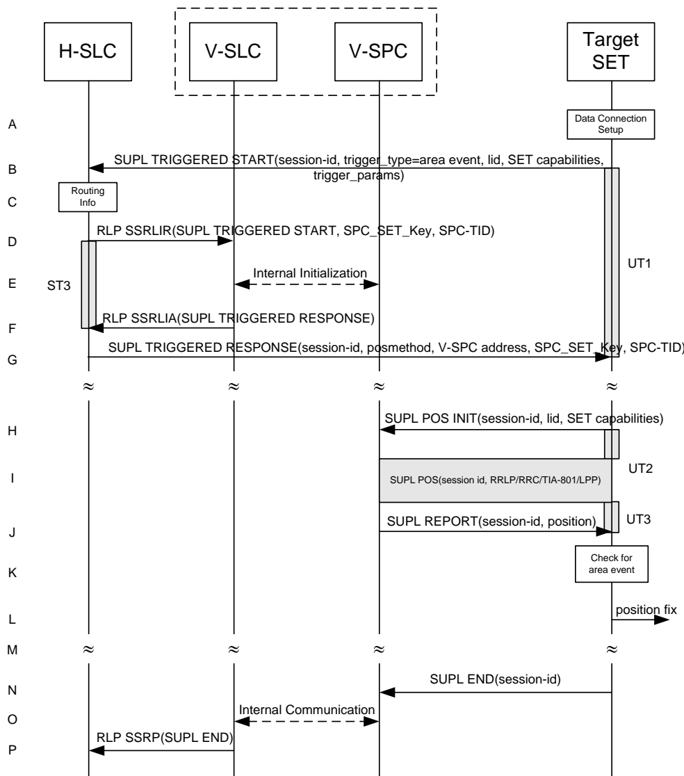
Figure 62: SET Initiated Area Event Trigger Service Roaming with V-SLP Positioning Successful Case – Non-Proxy Mode
