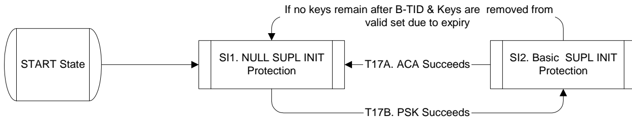
Figure 104: SUPL INIT Protection Level state transitions for the SET. Triggers T17A and T17B are sent from the Security Negotiation Model as described in section E.2.1.
