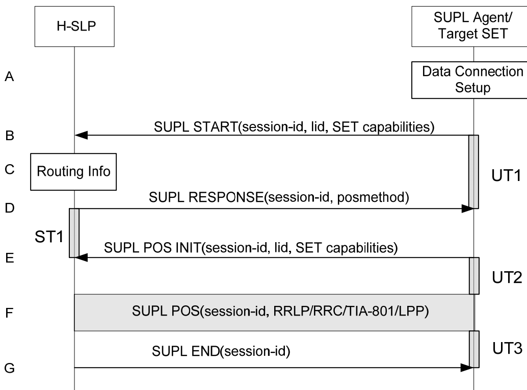
Figure 45: SET-Initiated Non-Roaming Successful Case - Proxy mode
