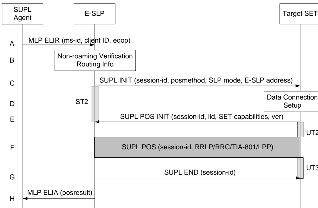
Figure 30: Network Initiated Emergency Services Non-Roaming Successful Case – Proxy Mode
