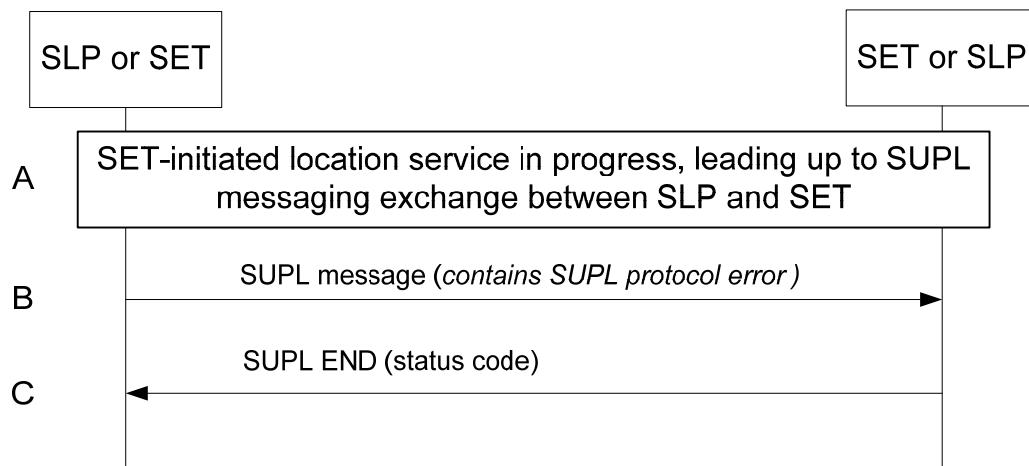
Figure 72: SET-Initiated Error SUPL Protocol Error
