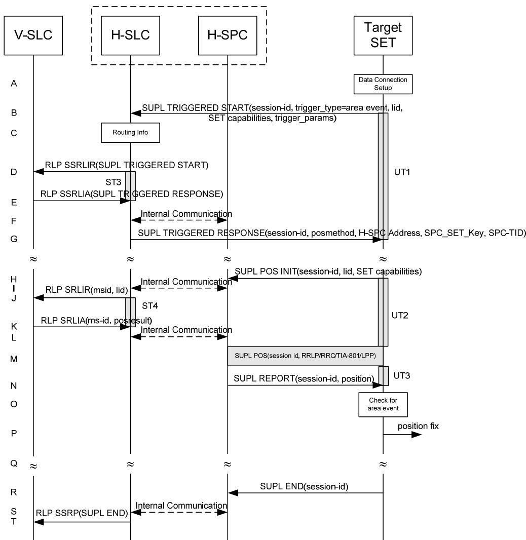
Figure 63: SET Initiated Area Event Trigger Service Roaming with H-SLP Positioning Successful Case – Non-Proxy Mode
