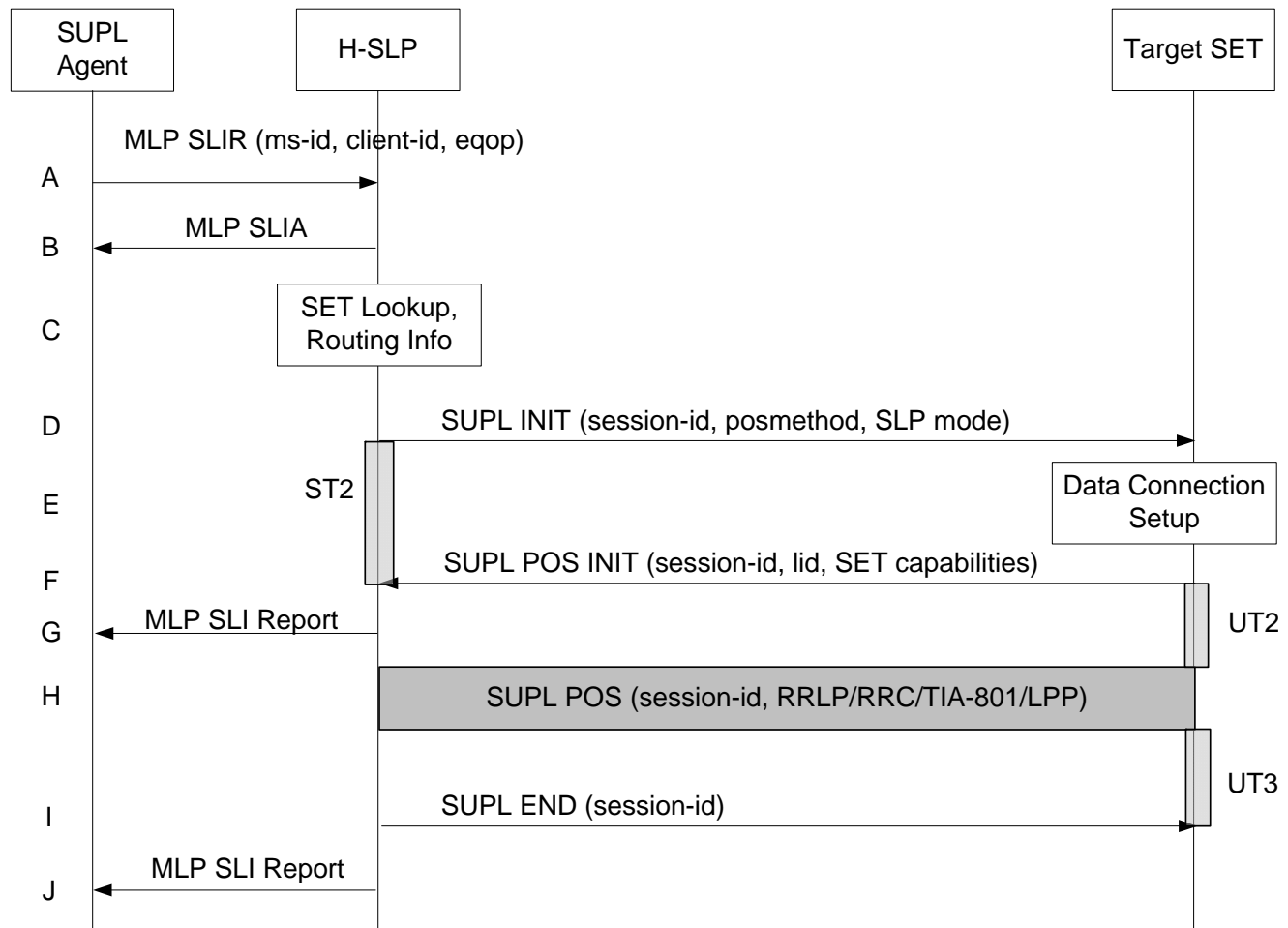
Figure 85: Network Initiated Non-Roaming Successful Case – Proxy Mode with asynchronous MLP request
