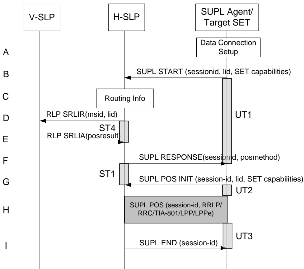
Figure 50: SET-Initiated Roaming with H-SLP Positioning Successful Case – Proxy mode
