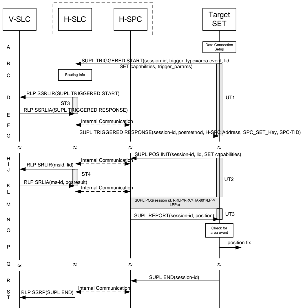
Figure 64: SET Initiated Area Event Trigger Service Roaming with H-SLP Positioning Successful Case – Non-Proxy Mode
