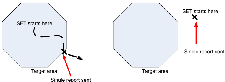
Figure 90: Single report when SET is outside area
