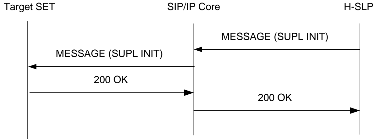
Figure 87: SIP Push Message flow
