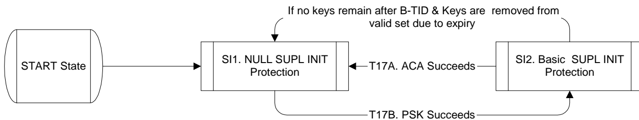
Figure 105: SUPL INIT Protection Level state transitions for the SET. Triggers T17A and T17B are sent from the Security Negotiation Model as described in section E.2.1.
