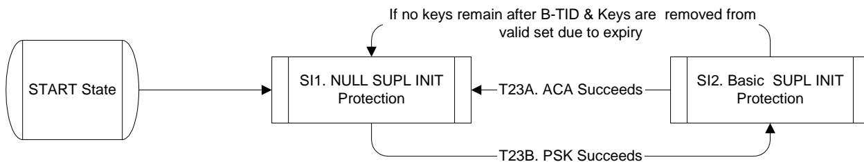
Figure 115: SUPL INIT Protection Level state transitions for the H-SLP. Triggers T23A and T23B are sent from the Security Negotiation Model as described in section E.3.1.
