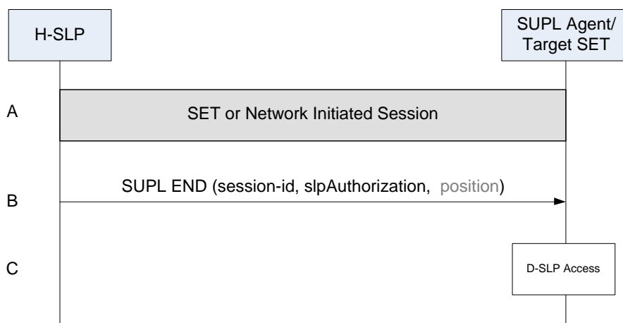
Figure 21: Unsolicited Authorization of D-SLPs by the H-SLP
