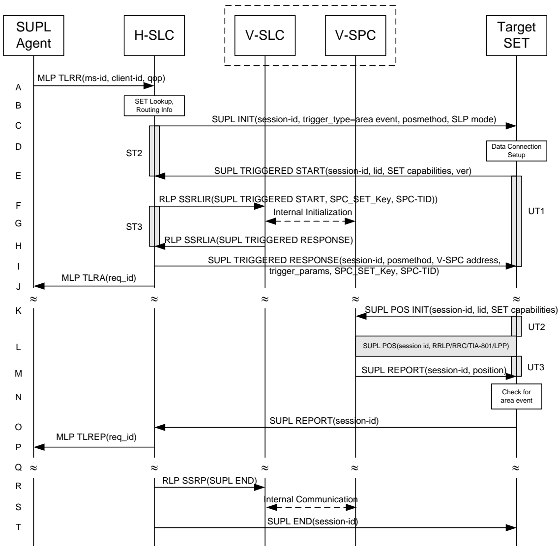
Figure 17: Network Initiated Area Event Trigger Service Roaming with V-SLP Positioning Successful Case – Non-Proxy Mode
