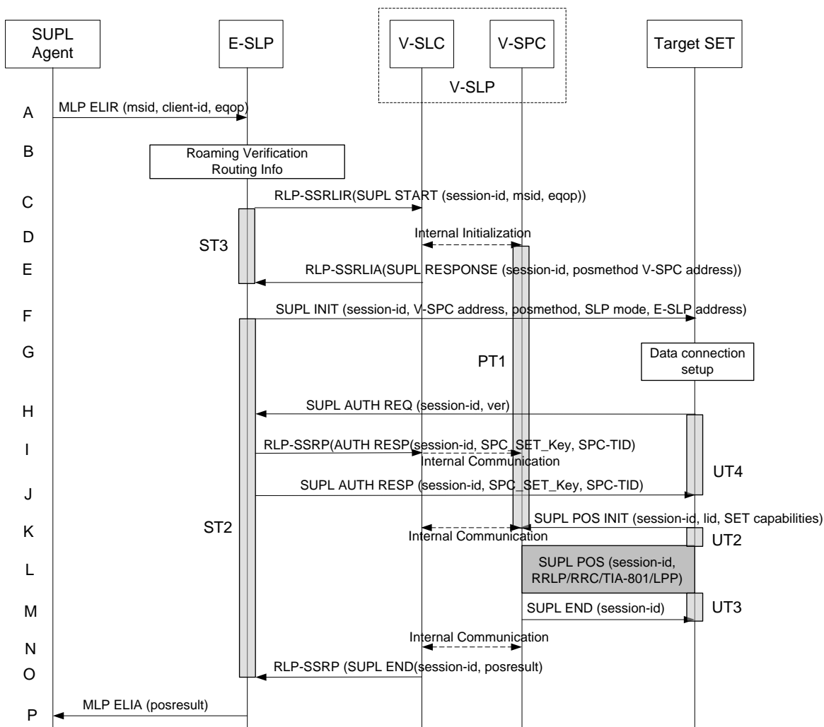
Figure 34: Network Initiated Emergency Services Roaming with V-SPC Positioning Successful Case – Non-Proxy-mode
