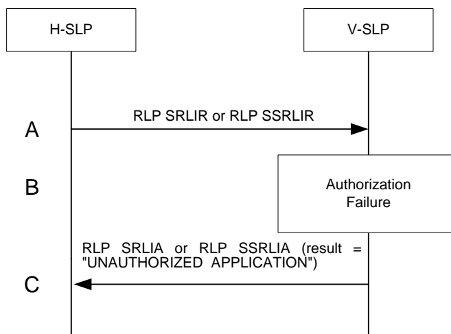
Figure 39: Network Initiated Authorization Failure V-SLP
