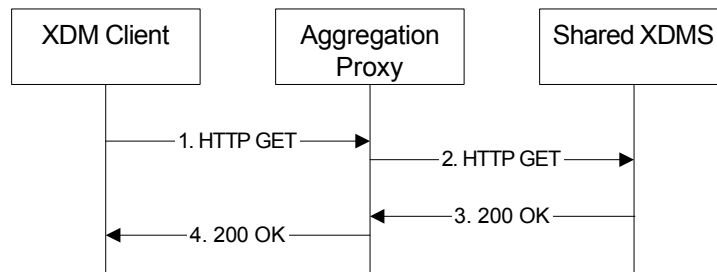
Figure B.1.2 XDM Client obtains Group Usage lists
