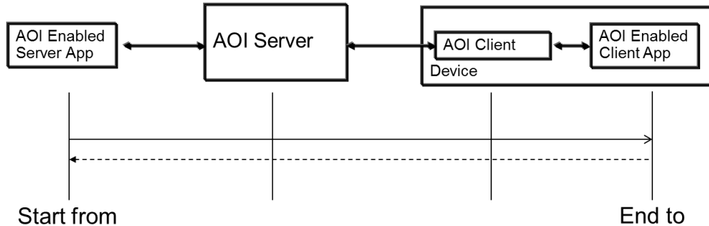
Figure 6: Notification Delivery Lifecycle
