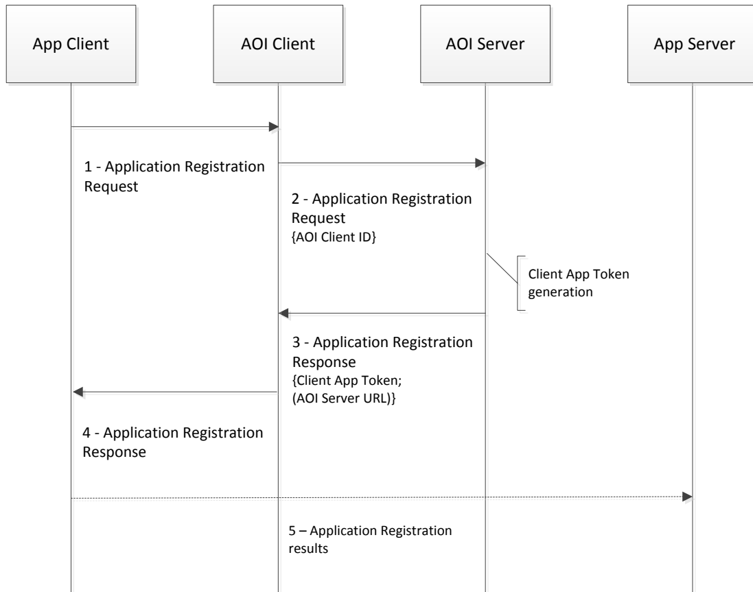
Figure 11: Client Application Registration
