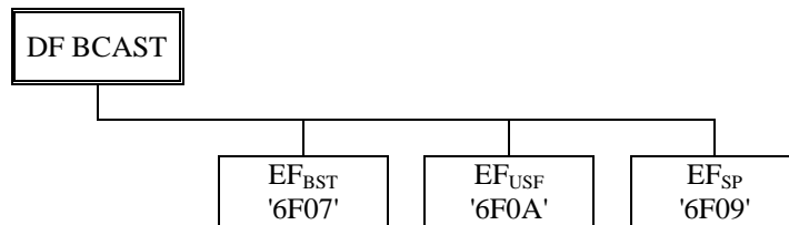
Figure 28 – File Identifiers of DF BCAST
