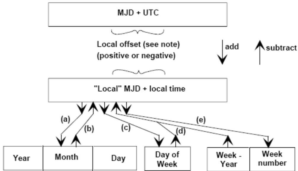
Figure 27 – Conversion routes between Modified Julian Date (MJD) and Co-ordinated Universal Time (UTC)
