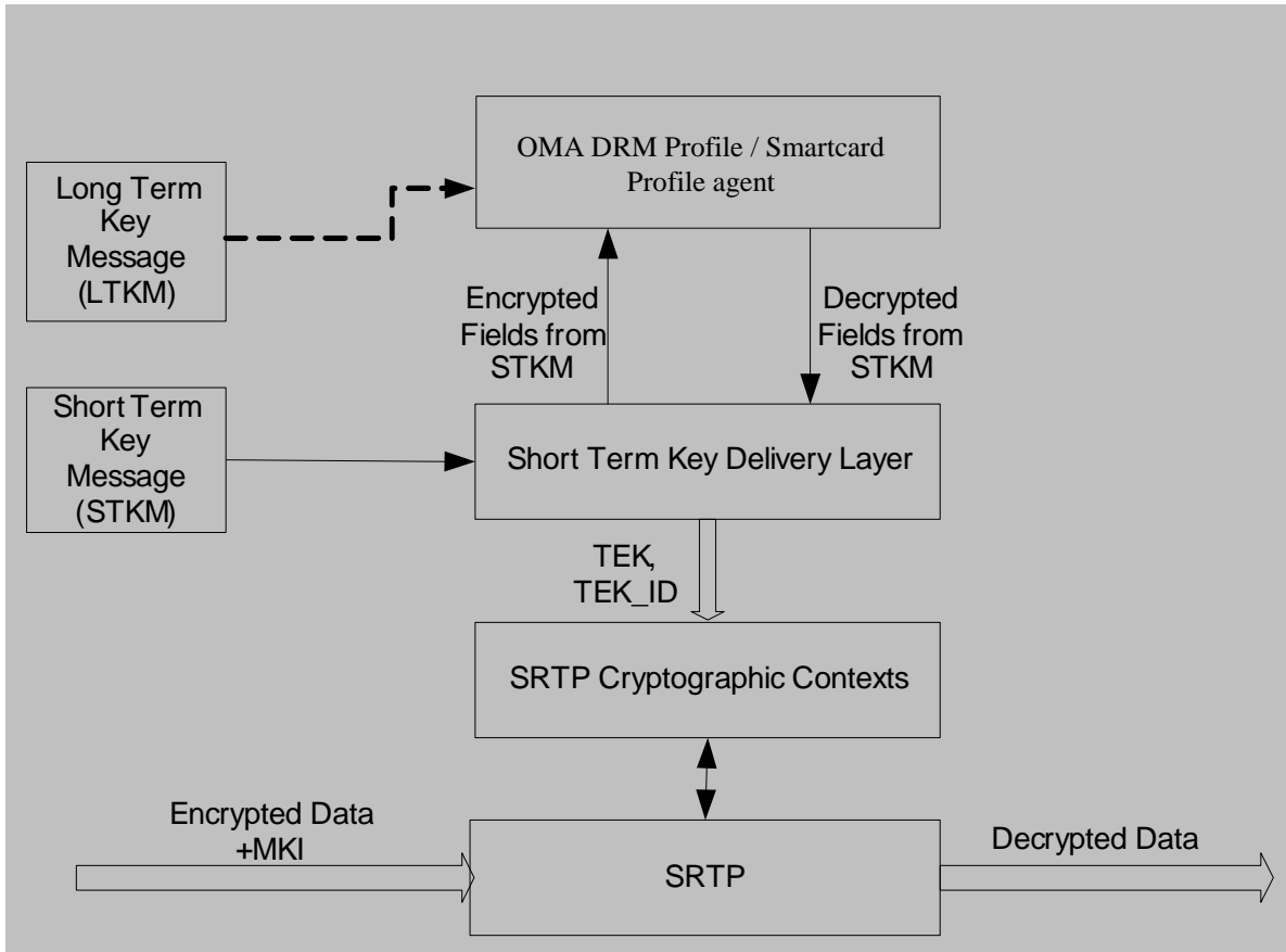
Figure 11 – SRTP Cryptographic Context Management (General Case)
