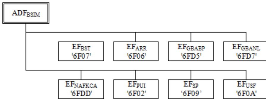
Figure 29 – File Identifiers and Directory Structures of BSIM
