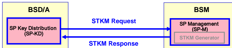
Figure 22 – Message Flow between BSD/A and BSM for Delivery STKMs
