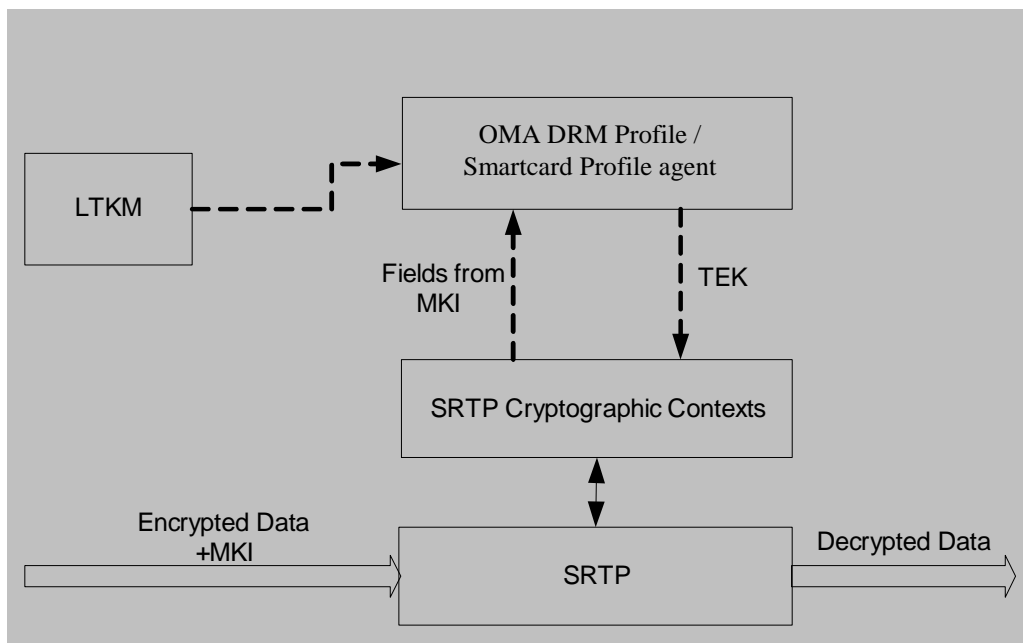
Figure 12 – SRTP Cryptographic Context Management (No Short Term Key Delivery Layer)
