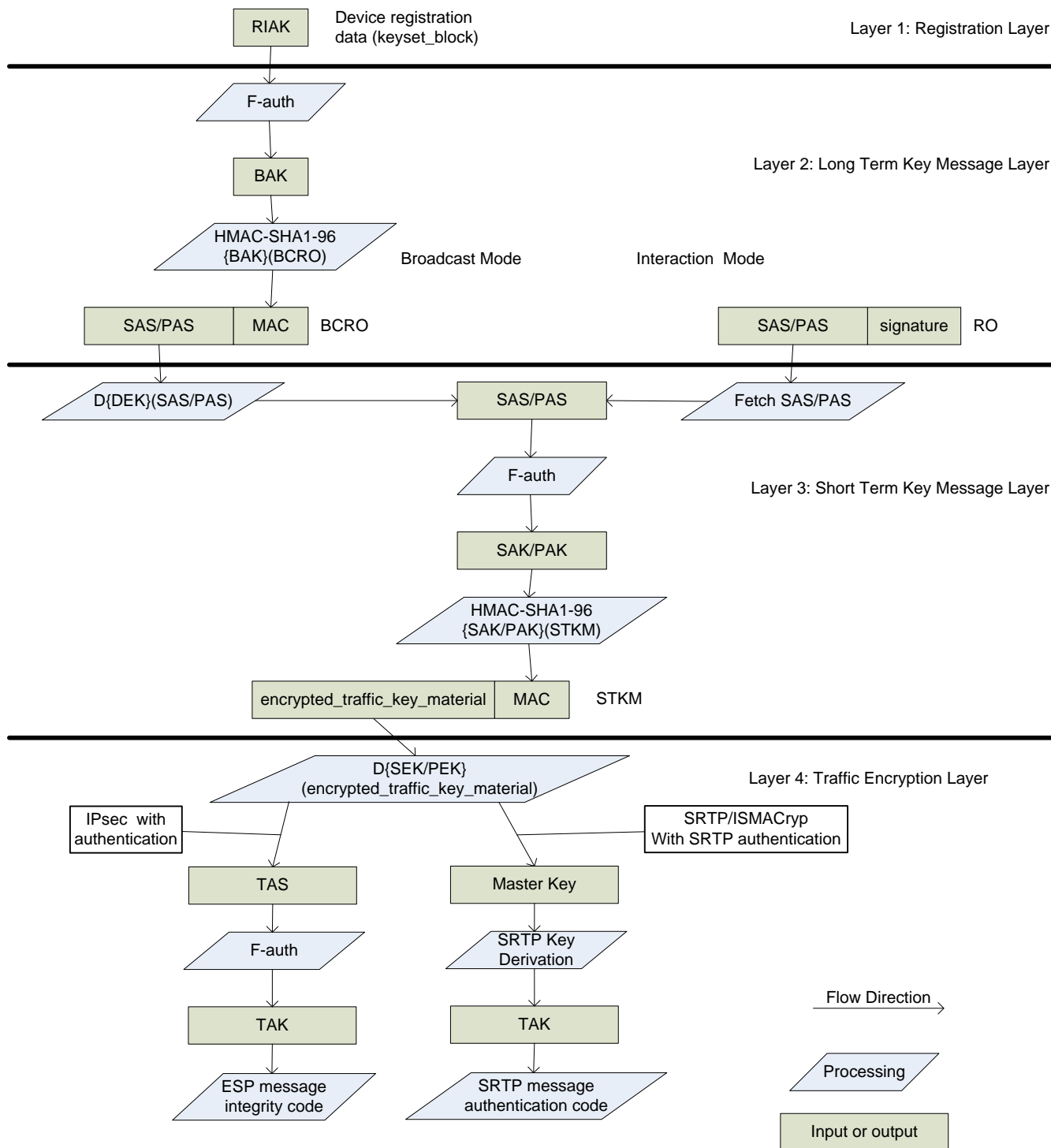
Figure 3: Authentication hierarchy
