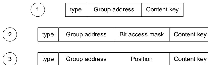
Figure 30: Addressing modes
