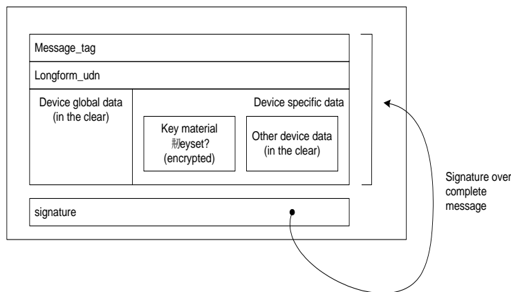
Figure 9: device_registration_response() message
