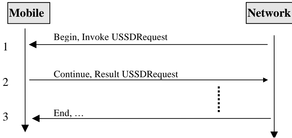
Figure 2. Network initiated USSD dialogue.
