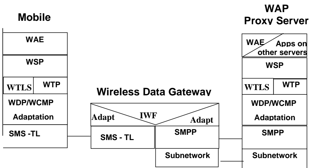
Figure 1.1 SMPP Tunnel in the WAP Architecture
