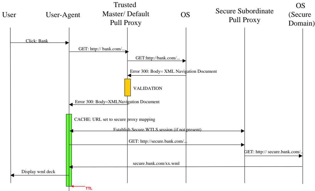
Figure 2: Sequence Diagram
