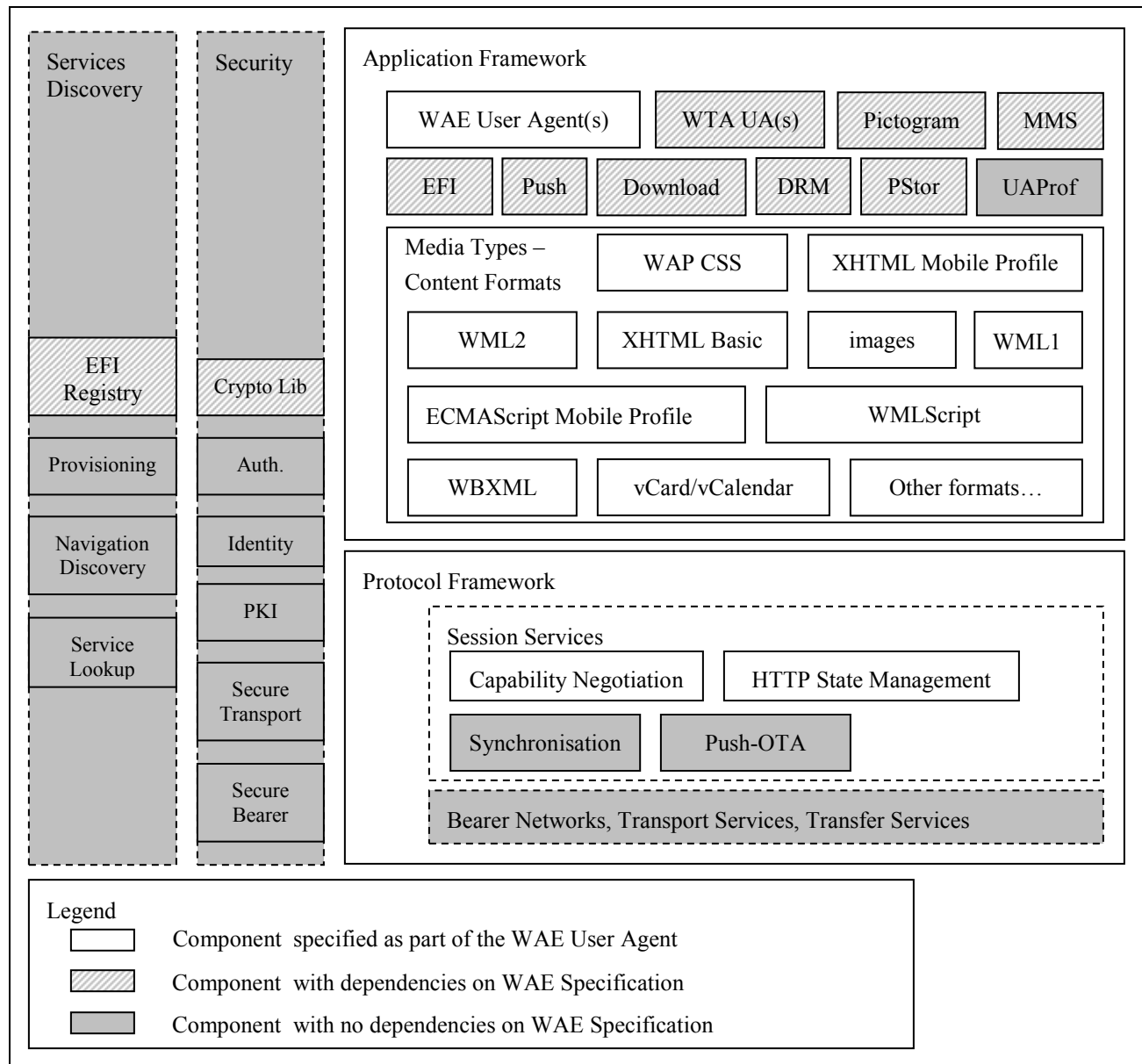
Figure 5-1: WAE Components in relation to the WAP version 2 architecture
