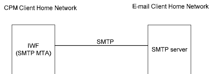
Figure 3 CPM to e-mail interworking architecture
