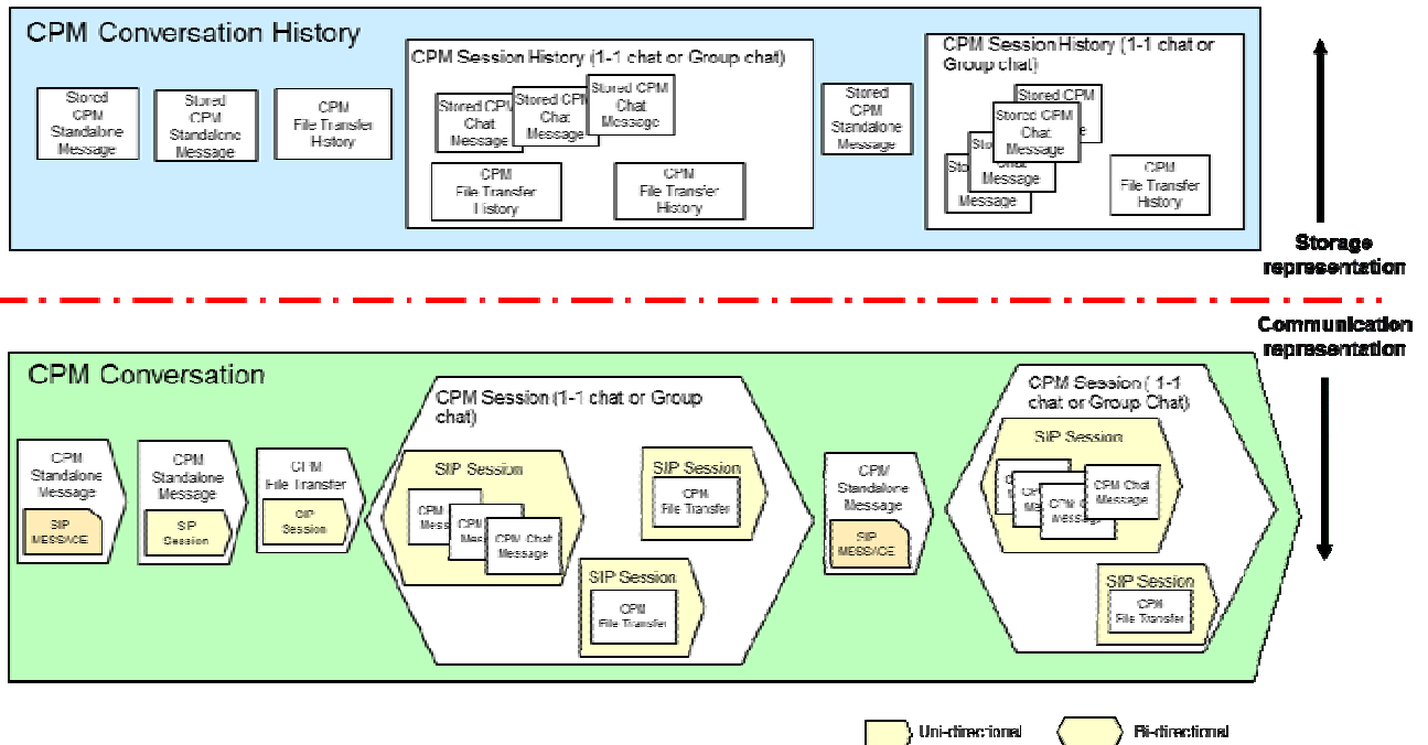
Figure 1: Illustration of the relationship between a CPM Conversation and a CPM Conversation History and depiction of the items they contain
