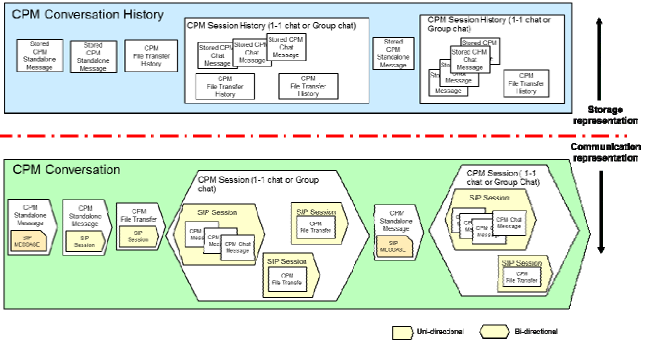
Figure 1: Illustration of the relationship between a CPM Conversation and a CPM Conversation History and depiction of the items they contain, a CPM Conversation is constituted by any number of CPM Standalone Messages, CPM File Transfers and CPM Sessions. A CPM Message is information of a discrete nature that can contain several discrete Media (e.g. text, images, audio-clips, video-clips). CPM Messages can be sent within a CPM Session (as a CPM Chat Message) or outside of a CPM Session (as a CPM Standalone Message), where a CPM Session represents a logical connection between CPM User and other Principal(s) established for a finite duration. A CPM File Transfer is a transfer of one or more files with multimedia contents between two Principals, in which the recipient Principal has to explicitly acknowledge the reception of the files before any data of the files is transferred. In a CPM Session, Principals can also exchange continuous Media, that due to the continuous nature of this type of information, need a logical connection (i.e. with a beginning and an end) to be set up and maintained between CPM User and other Principals. An underlying assumption is that a CPM Conversation should only be composed of one CPM Session at a given time. A user could however participate in several CPM Conversations in parallel (each of them containing one CPM Session) but this is not the intent of this diagram to show that functionality.
