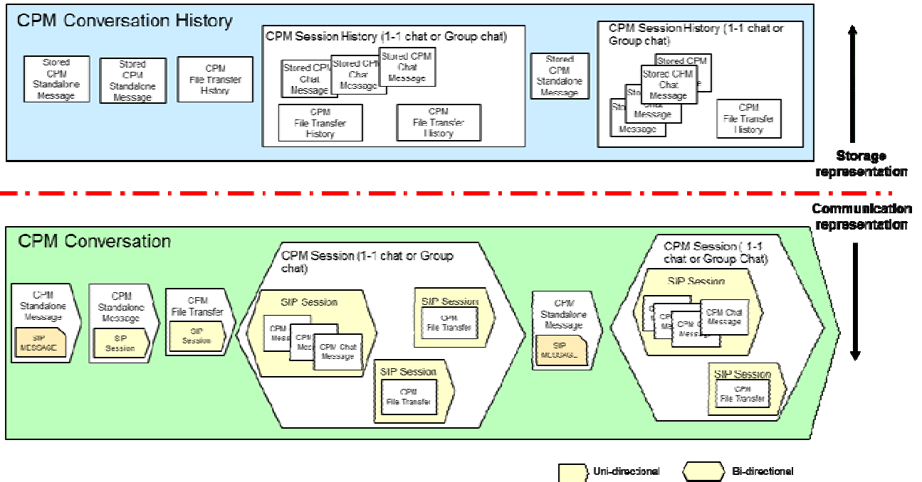
Figure 1: Illustration of the relationship between a CPM Conversation and a CPM Conversation History and depiction of the items they contain capture the potential of a CPM Conversation and a CPM Conversation History respectively, and the relationship between them.
