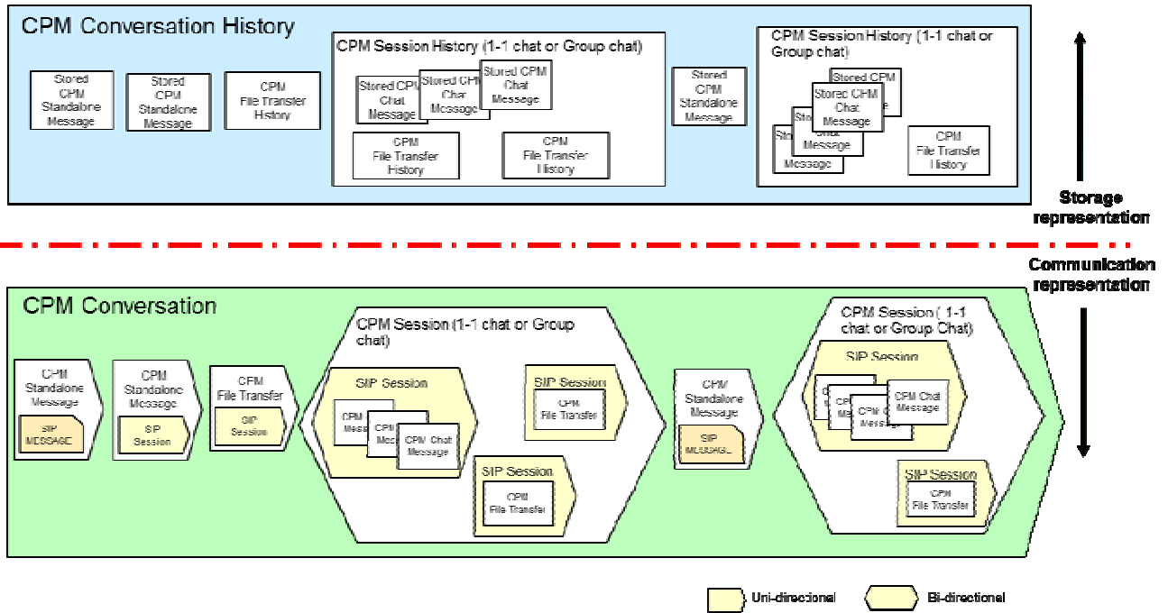
Figure 1: Illustration of the relationship between a CPM Conversation and a CPM Conversation History and depiction of the items they contain. Authorized Principals can capture and store the information that they have been exchanging during a CPM Conversation as a CPM Conversation History in network-based storage provided by a CPM service provider. As such, a CPM Message may become a stored CPM Message, a CPM File Transfer may become a CPM File Transfer History and continuous Media may become stored Media (e.g. voice-clip, video-clip). When stored CPM Chat Messages and stored Media are part of the same CPM Session, they are associated together in network based storage as a CPM Session History. Stated in another manner, a CPM Conversation History can be described as CPM Session Histories, CPM File Transfer Histories and stored CPM Standalone Messages, derived respectively from the CPM Sessions and any CPM File Transfers and CPM Standalone Messages exchanged outside a CPM Session during a CPM Conversation.
