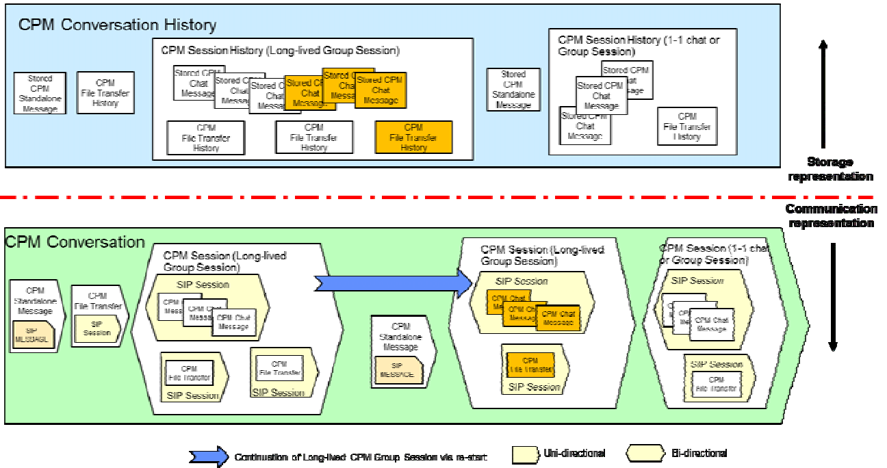
Figure 3: Illustration of the relationship between a CPM Conversation and a CPM Conversation History containing a Long-lived CPM Group Session, CPM 2.0
