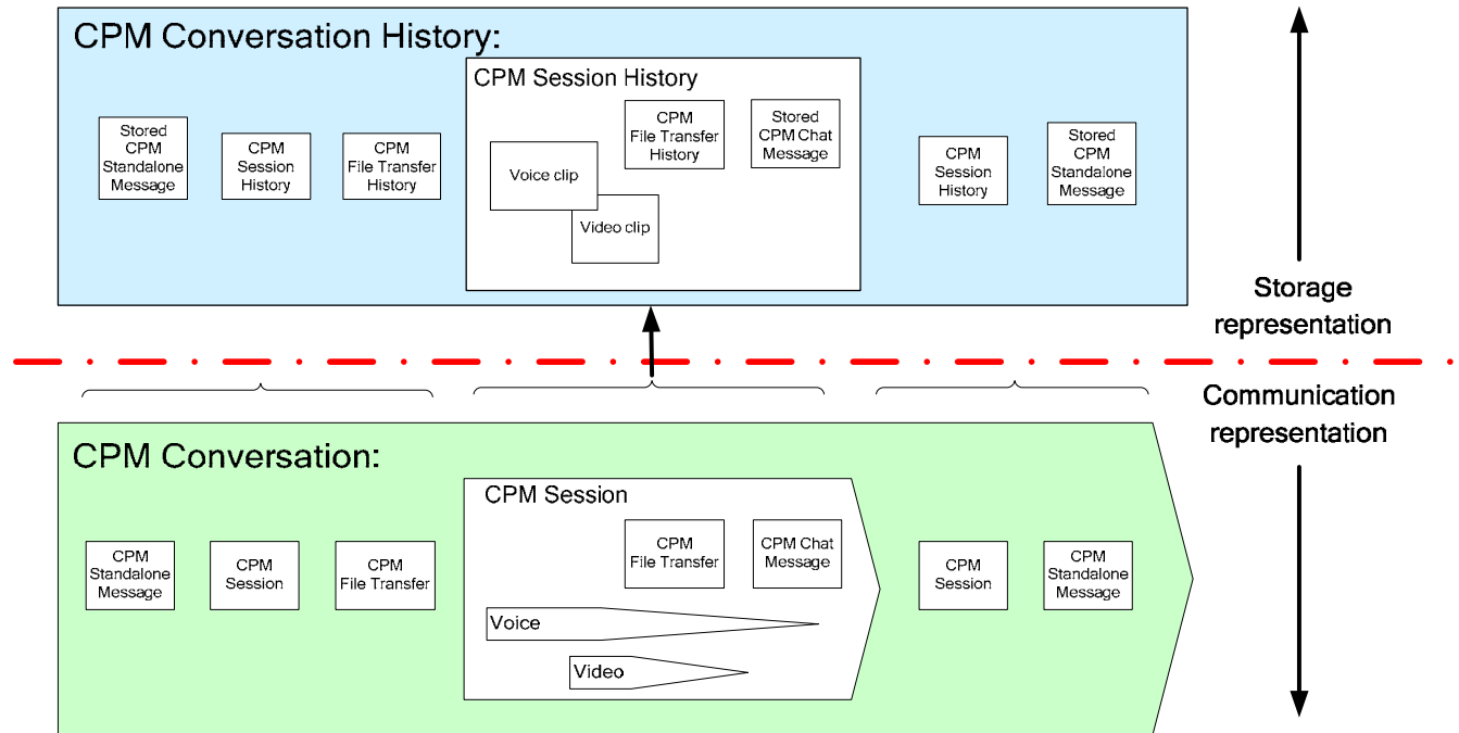
Figure 2: Illustration of the relationship between a CPM Conversation and a CPM Conversation History and depiction of the items they contain, CPM 1.0
