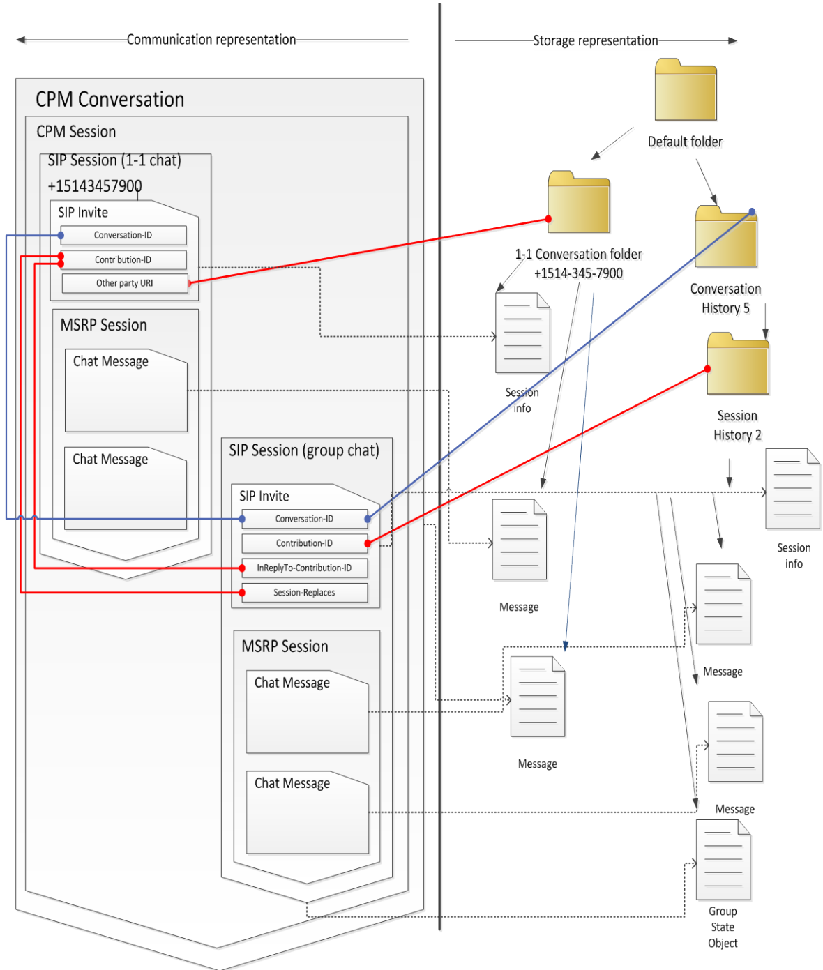
Figure 5: Example of storage representation; extending 1-1 chat to group chat
