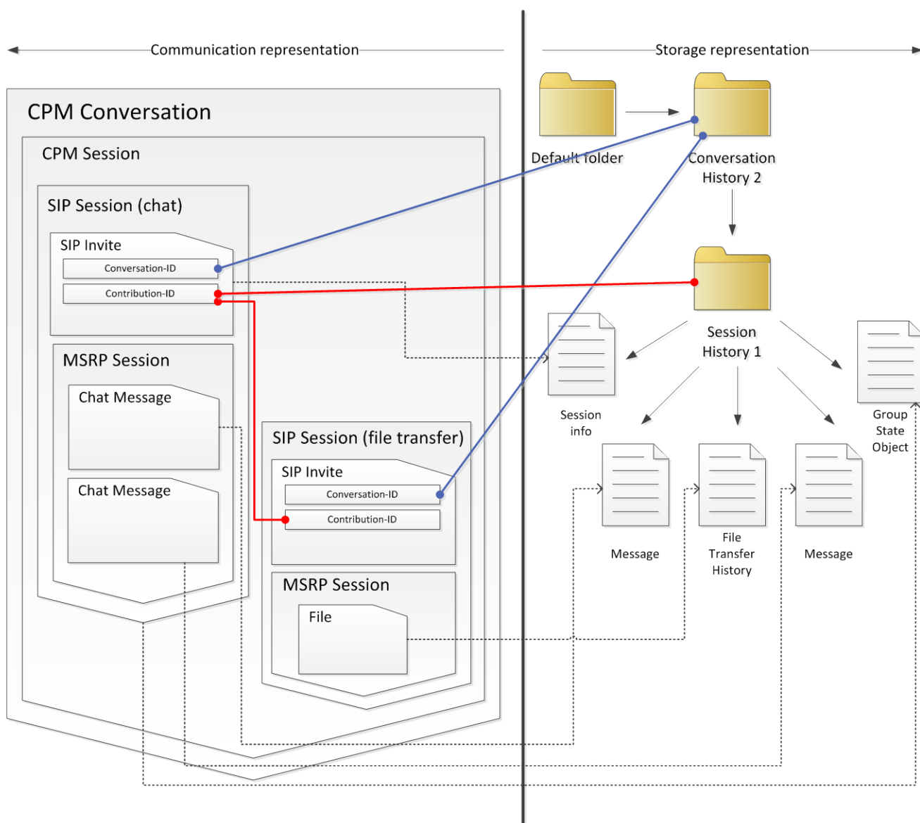
Figure 2: Example of storage representation; chat exchanges
