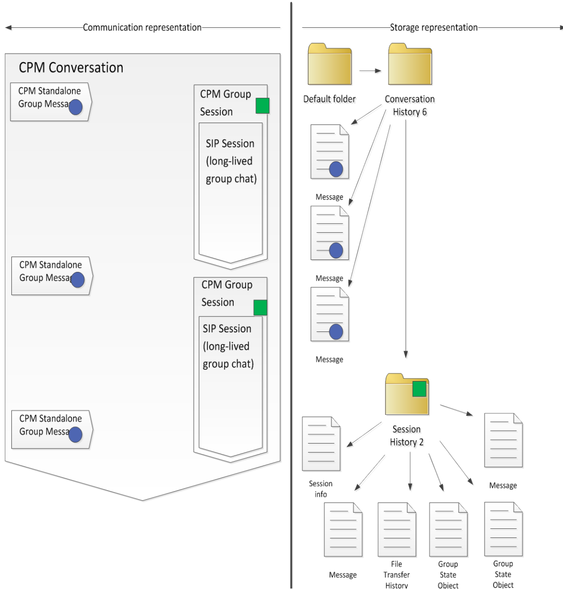
Figure 6: Example of storage representation; conversation via parallel channels
