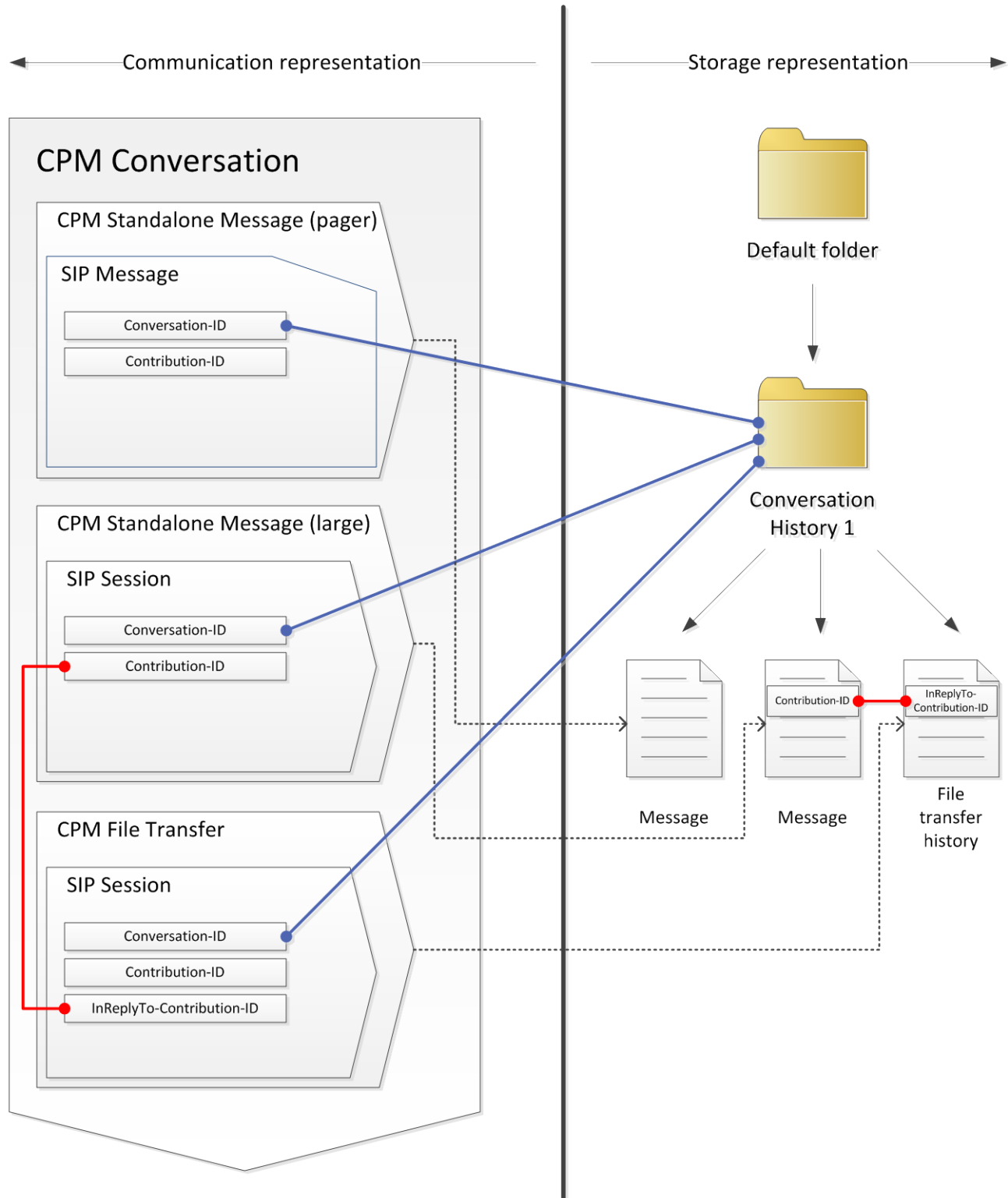
Figure 1: Example of storage representation; standalone exchanges
