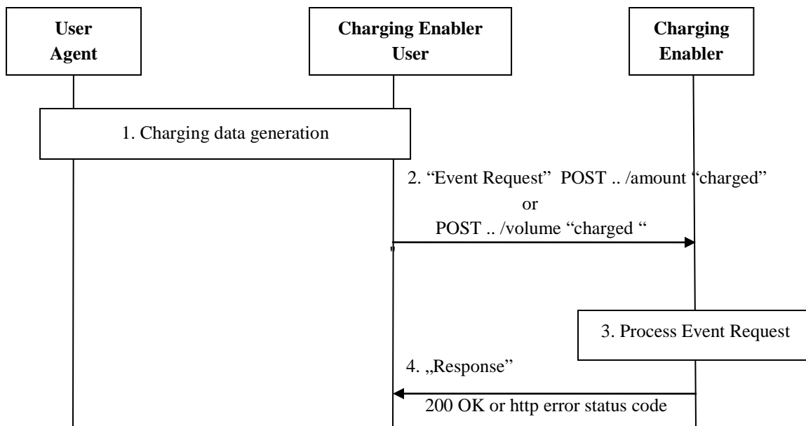
Flow 4: Event-based Offline Charging with REST binding
