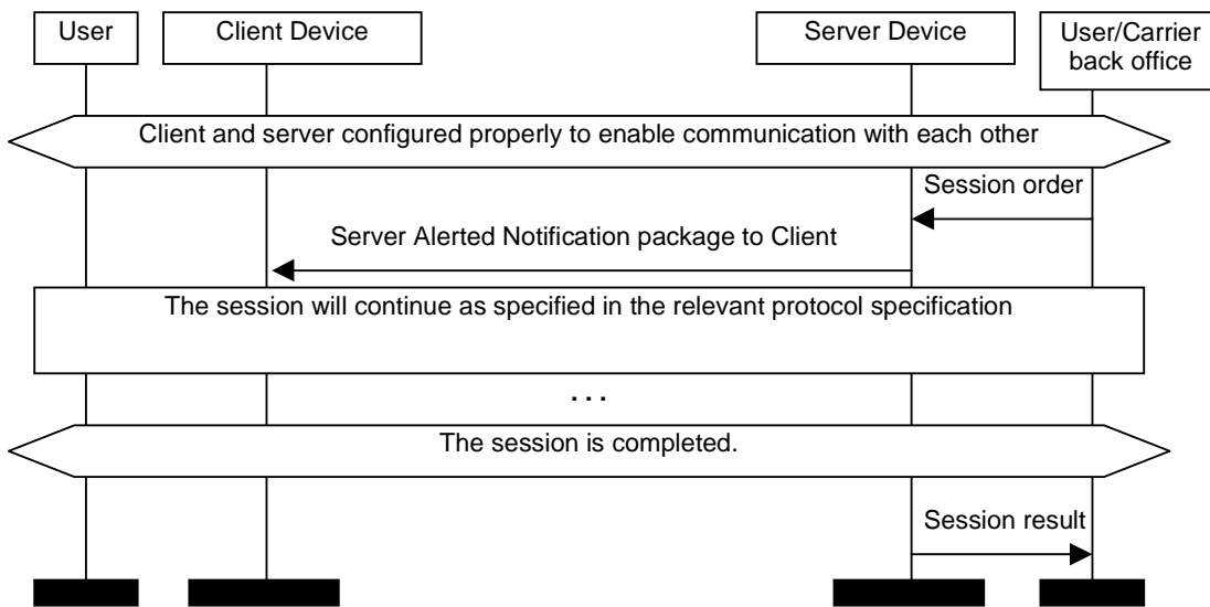
Figure 1. MSC of the Server Alerted Notification session
