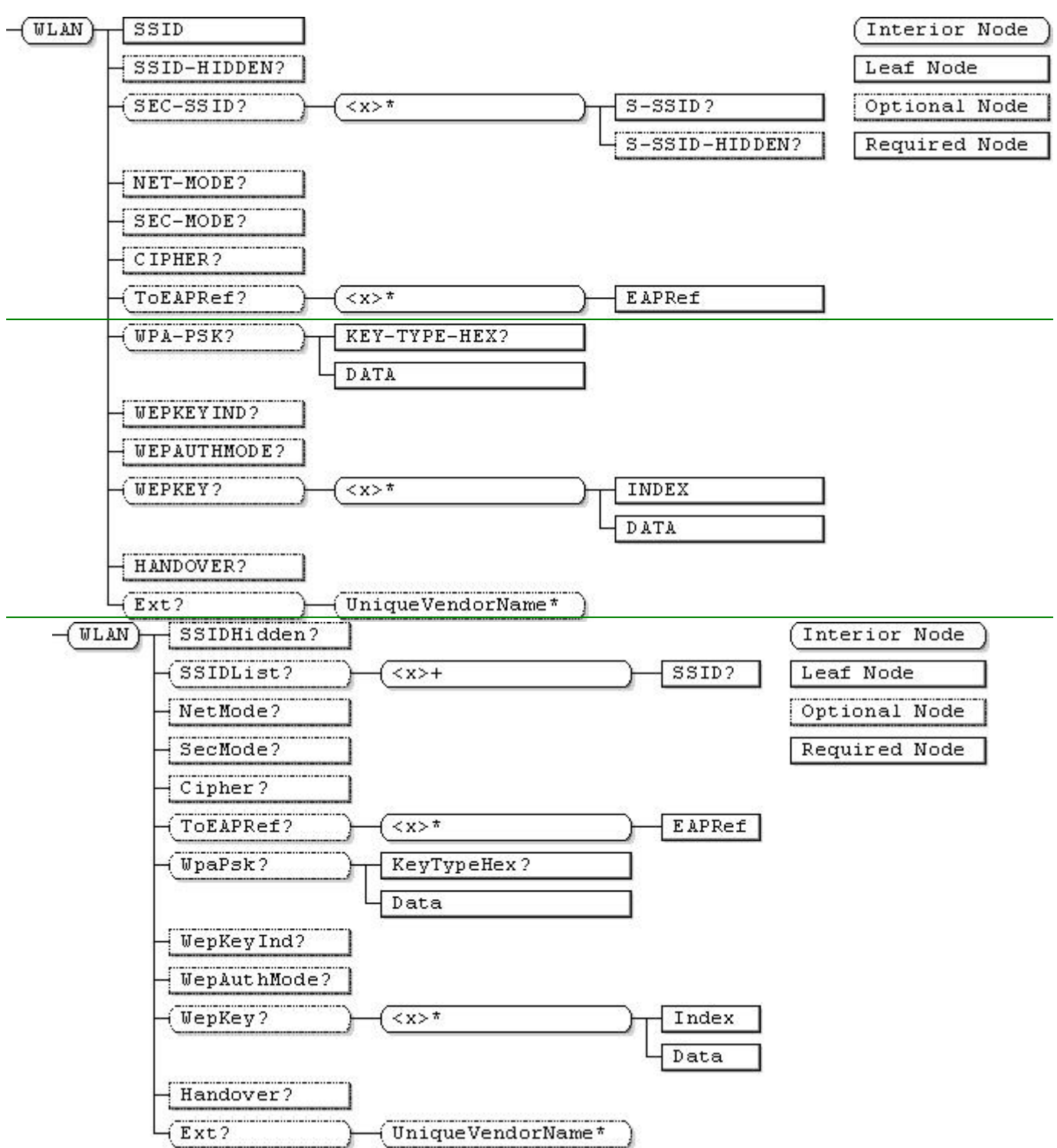
Figure 1. WLAN Management Object
