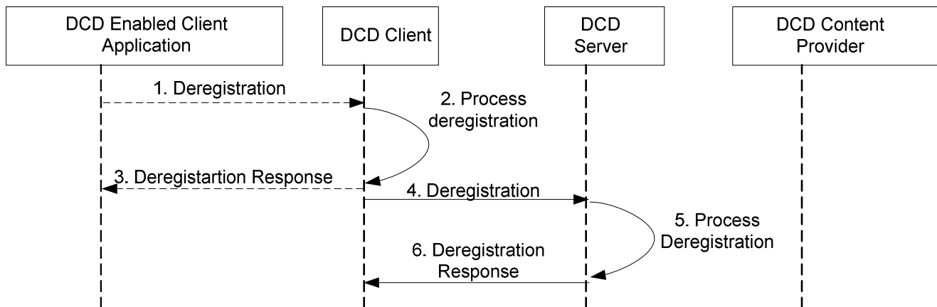
Figure 13: Deregistration of DCD Enabled Client Application
