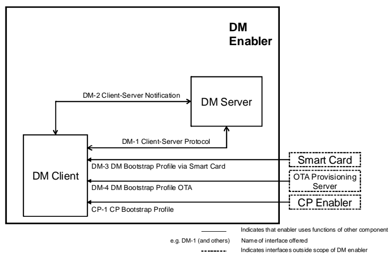
Figure 1: Device Management Architecture using interfaces
