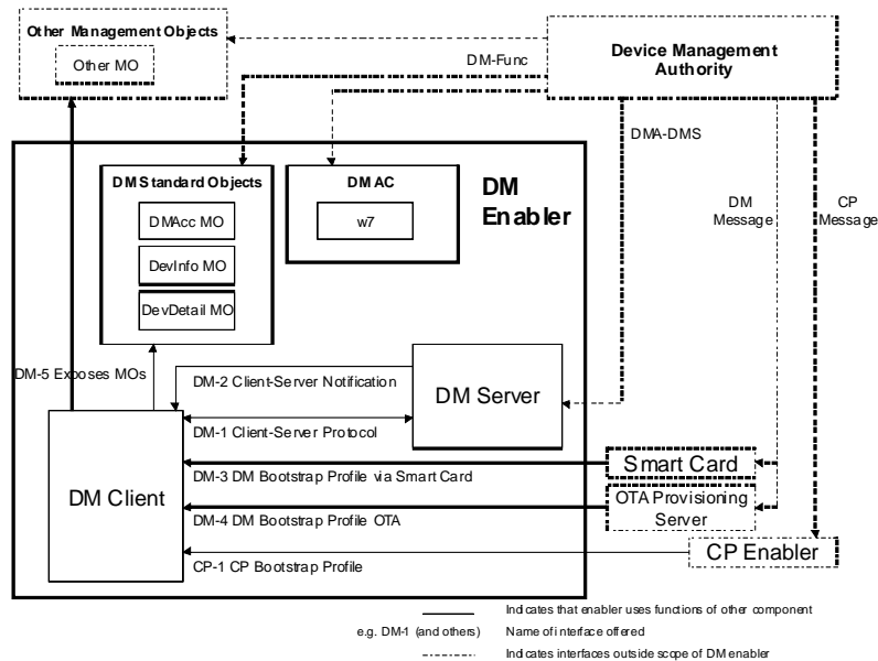
Figure 2: Device Management Architecture using interfaces
