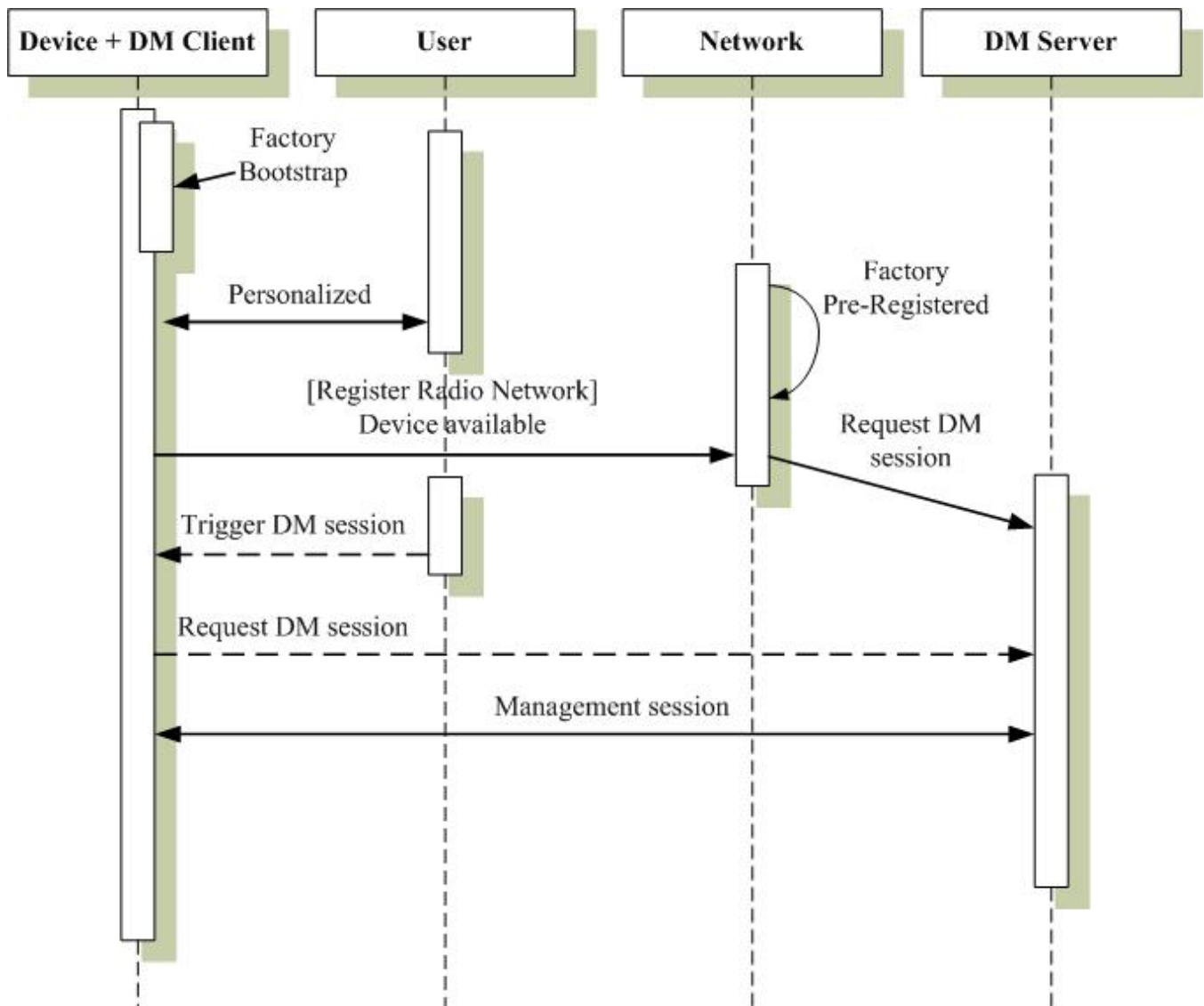
Figure 1: Customized bootstrap
