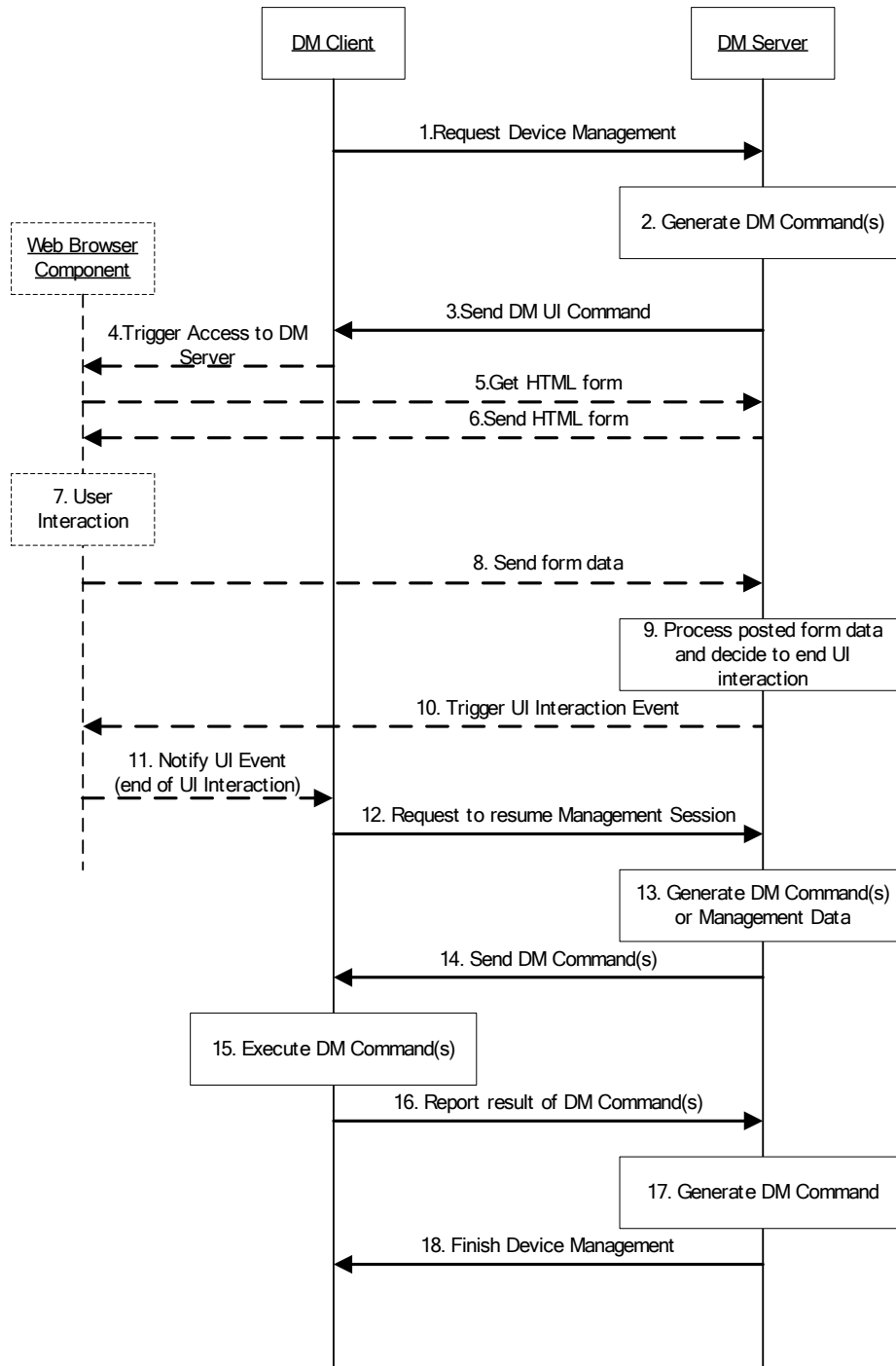
Figure 4: UI Interaction with Web Browser Call Flow
