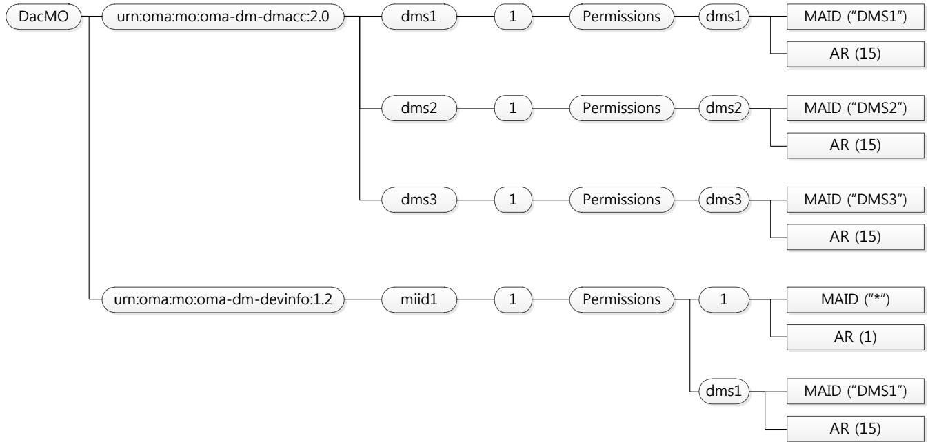
Figure 17: Examples for Delegation Access Control MO
