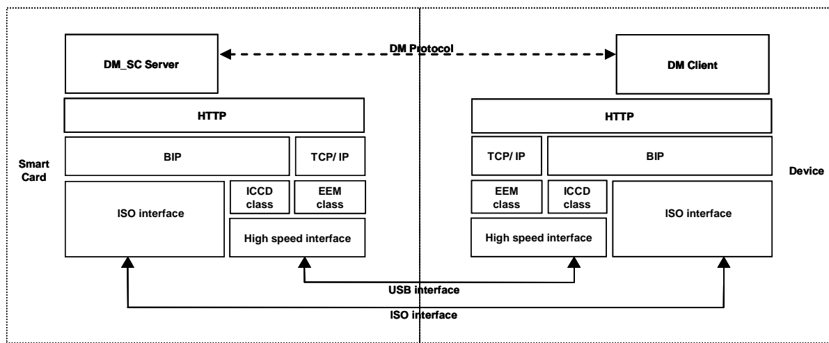
Figure 1: DM_SC Model
