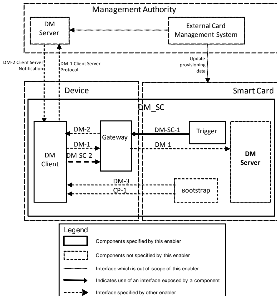
Figure 2: Architecture using interfaces
