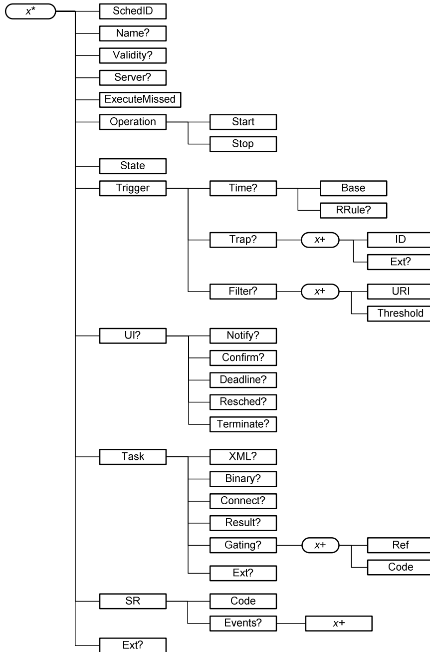
Figure 2: Scheduling Management Objects
