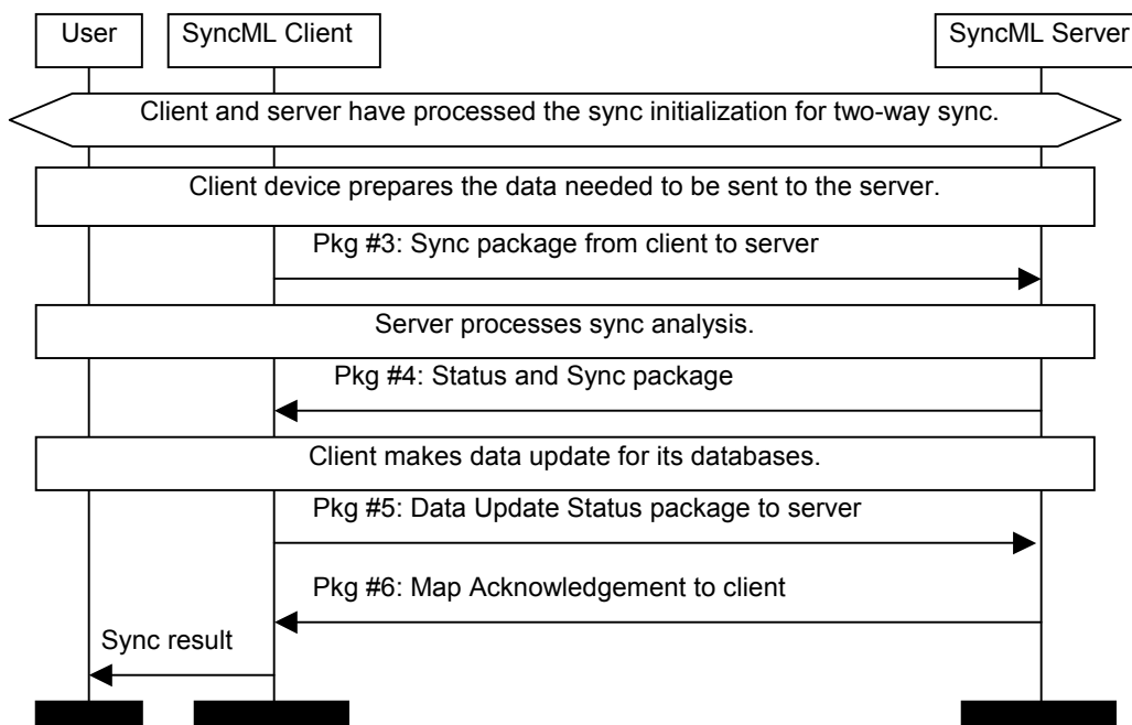
Figure 8 MSC of Two-Way Sync
