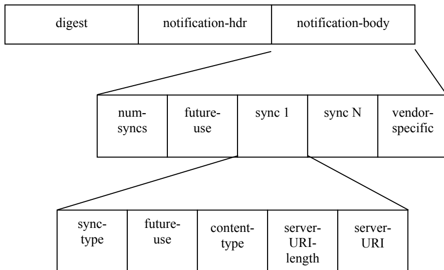
Figure 11. Format of the Server Alerted Sync Package (Pkg #0)
