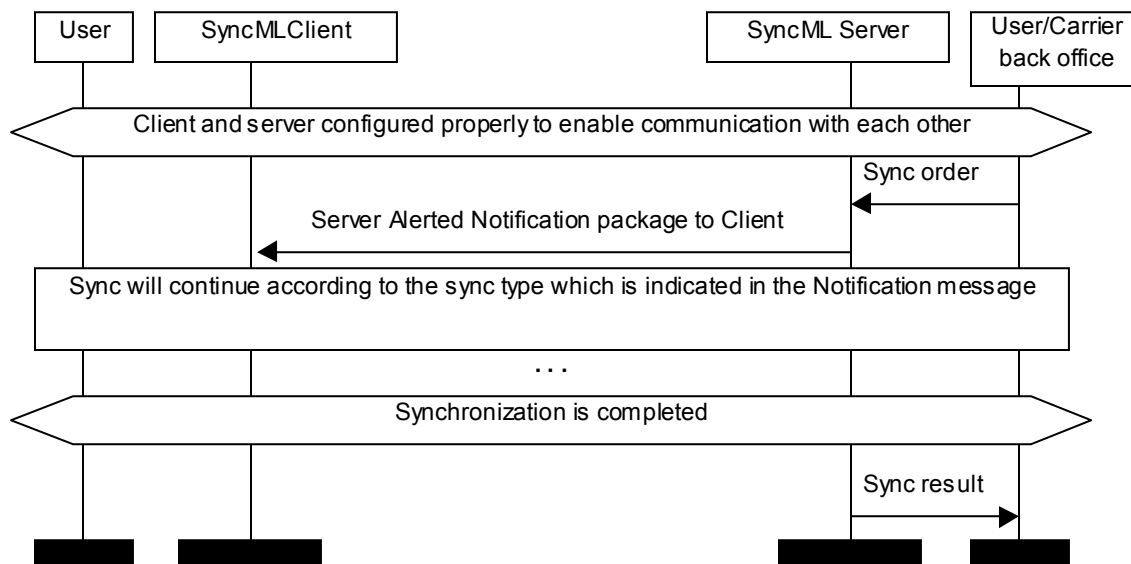
Figure 10. MSC of the Server Alerted Sync session
