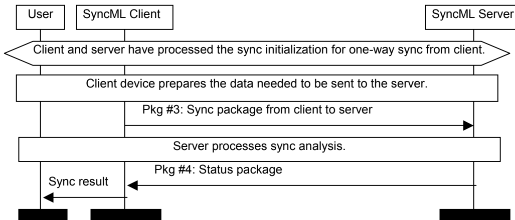
Figure 9 MSC of One-Way Sync from Client only
