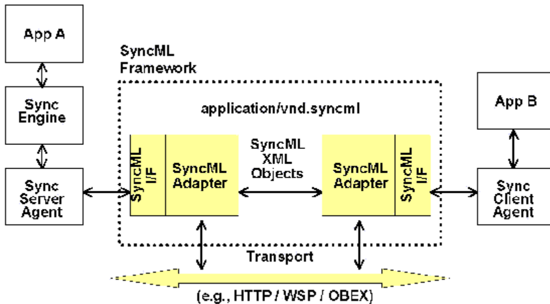
Figure 2 SyncML Framework
