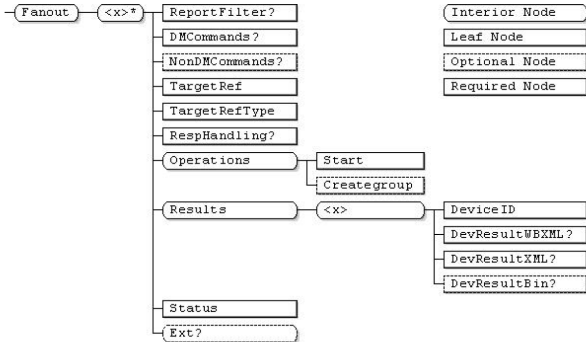
Figure 4: Fanout MO
