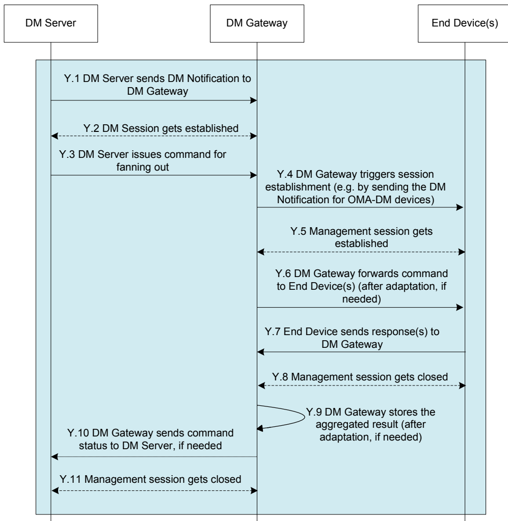
Figure 8: Synchronous Management in Proxy/Adaptation Mode
