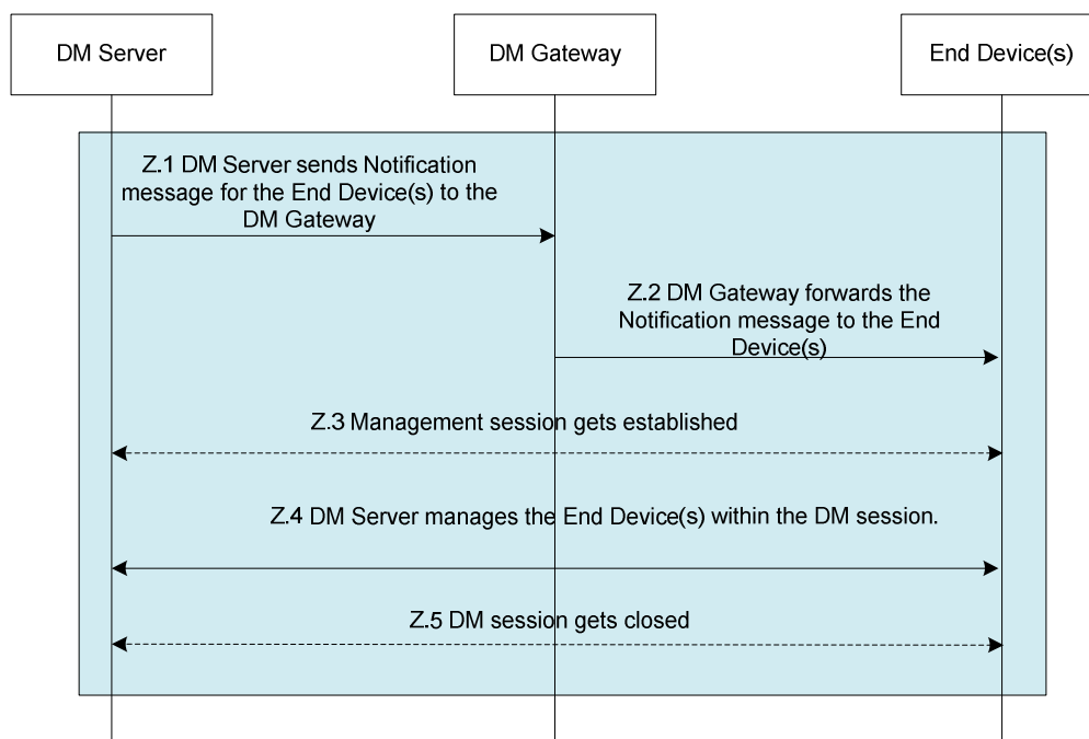
Figure 10: Management Flow in Transparent Mode
