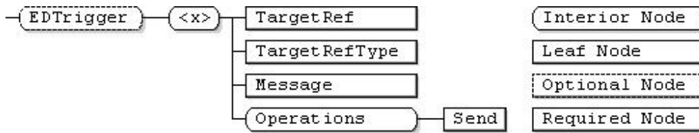
Figure 6: End Device Trigger MO
