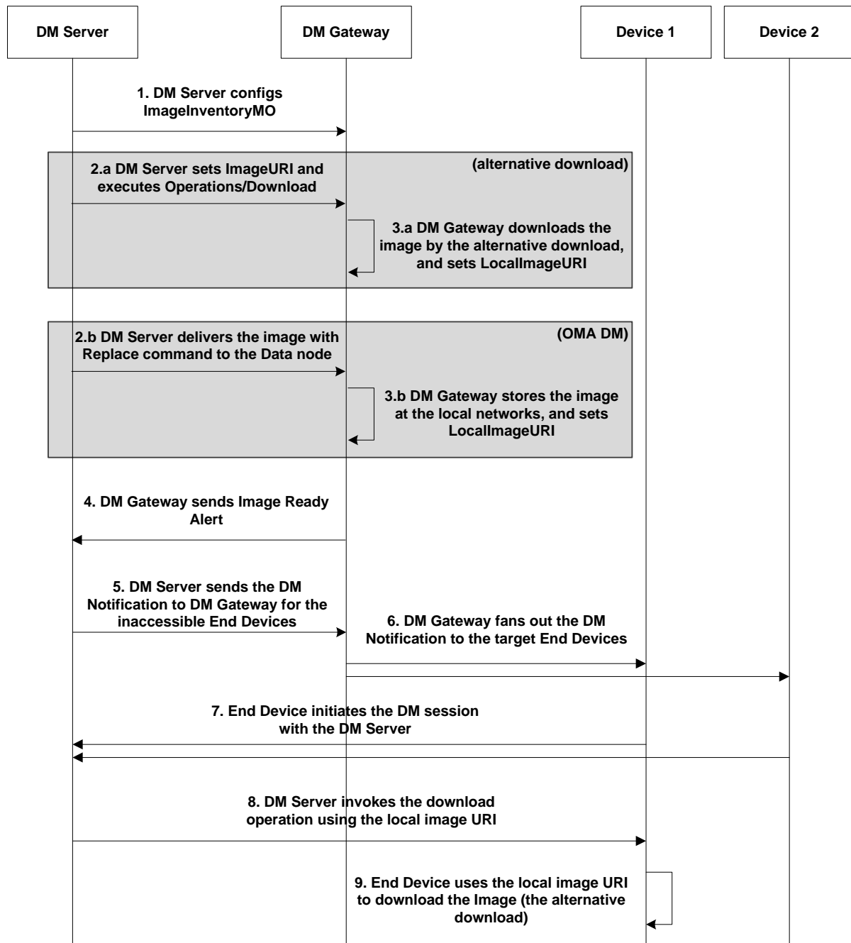
Figure 22: Image Distribution in Transparent Mode
