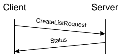
Figure 18. Create contact list transaction
