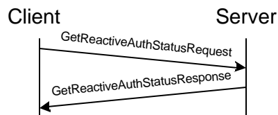
Figure 32. Get reactive authorization status transaction
