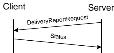
Figure 41. Delivery Status Report Transaction
