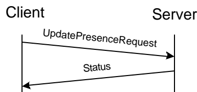
Figure 33. Update presence transaction
