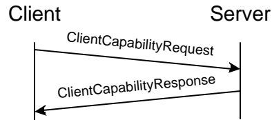
Figure 10. Client Capability Request
