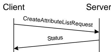
Figure 21. Create attribute list transaction
