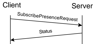
Figure 24. Subscribe presence transaction
