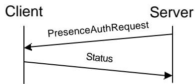
Figure 29. Reactive presence authorization request transaction
