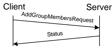
Figure 54. Add group members transaction
