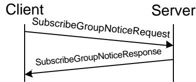
Figure 60. Subscribe group change notification transaction
