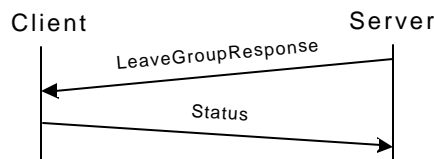
Figure 51. Server initiated leave group transaction
