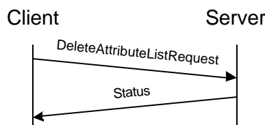
Figure 22. Delete attribute list transaction
