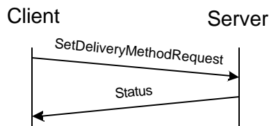
Figure 35. Set Delivery Method transaction
