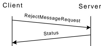
Figure 37. Reject Message transaction
