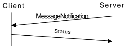
Figure 39. Message Notification transaction
