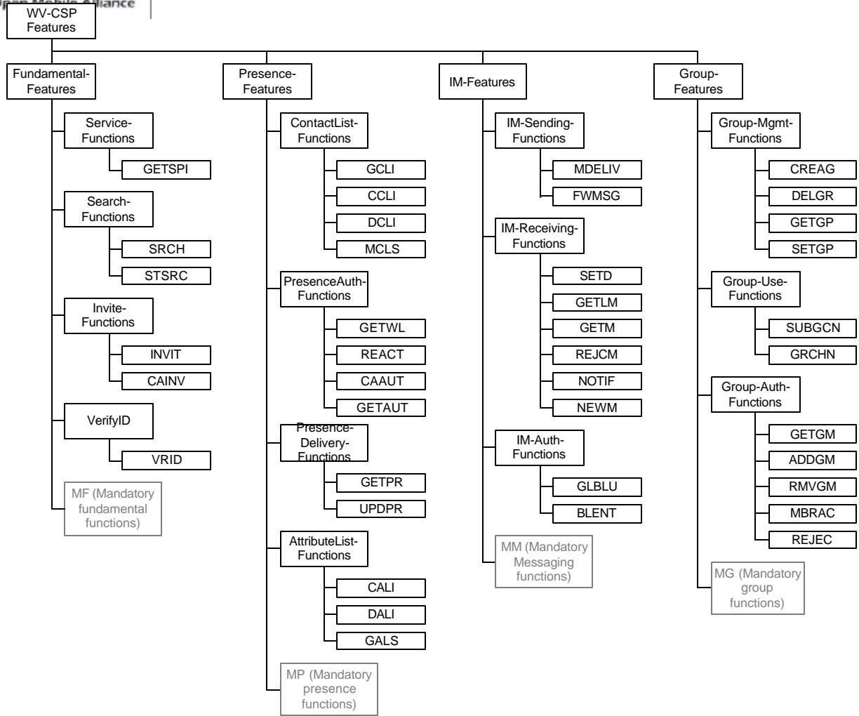
Figure 9. The service tree
