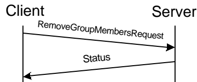
Figure 55. Remove group members transaction
