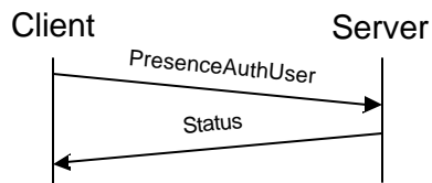
Figure 30. Reactive presence authorization of user transaction
