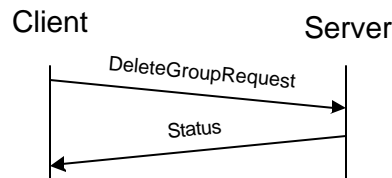
Figure 47. Delete group transaction
