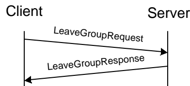
Figure 50. User initiated leave group transaction
