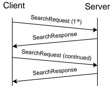
Figure 11. General search transactions
