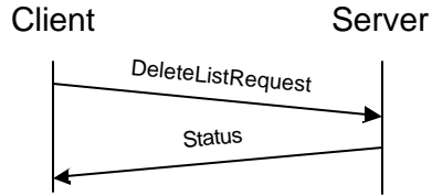
Figure 19. Delete contact list transaction
