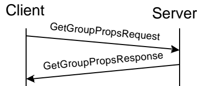
Figure 57. Get group properties transaction
