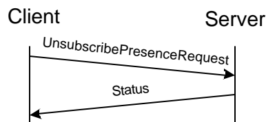
Figure 25. Unsubscribe presence transaction
