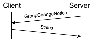
Figure 61. Group change notification
