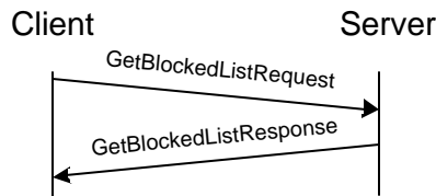
Figure 44. Get list of blocked entities transaction
