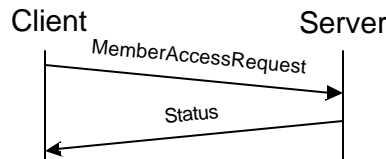
Figure 56. Member access rights transactions
