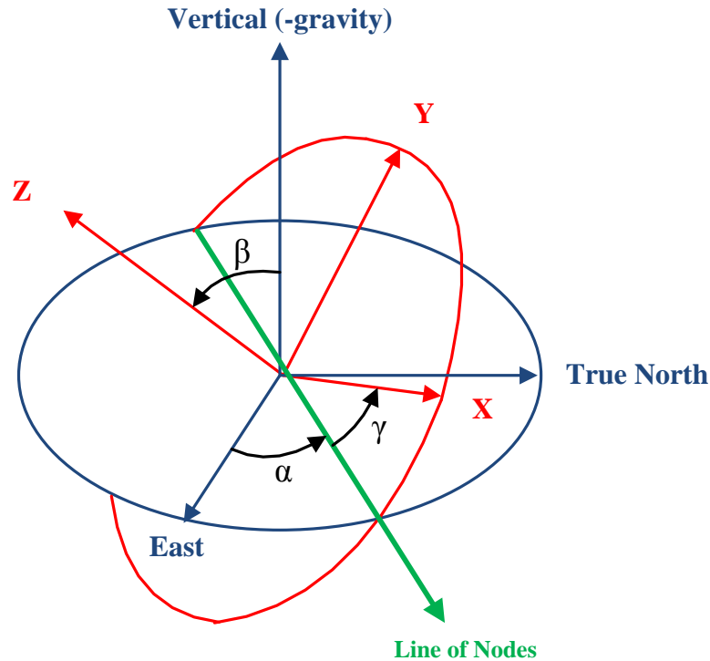
Figure 16: Euler Angles
