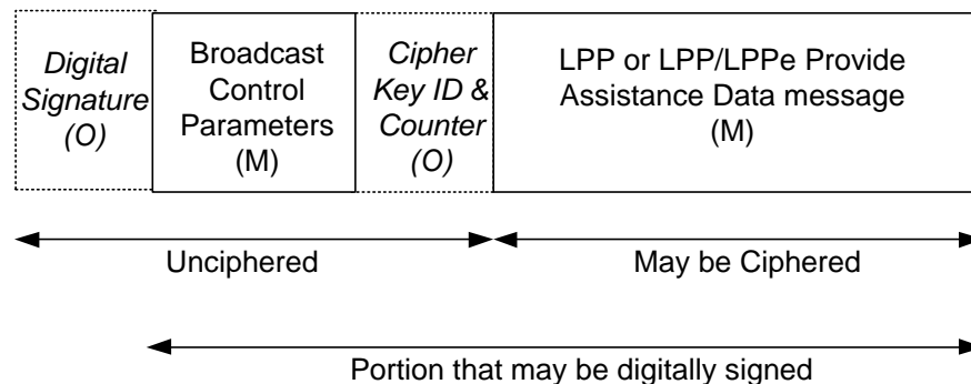
Figure 12: An encapsulated LPP/(LPPE) Broadcast Message with Mandatory (M) and Optional (O) portions
