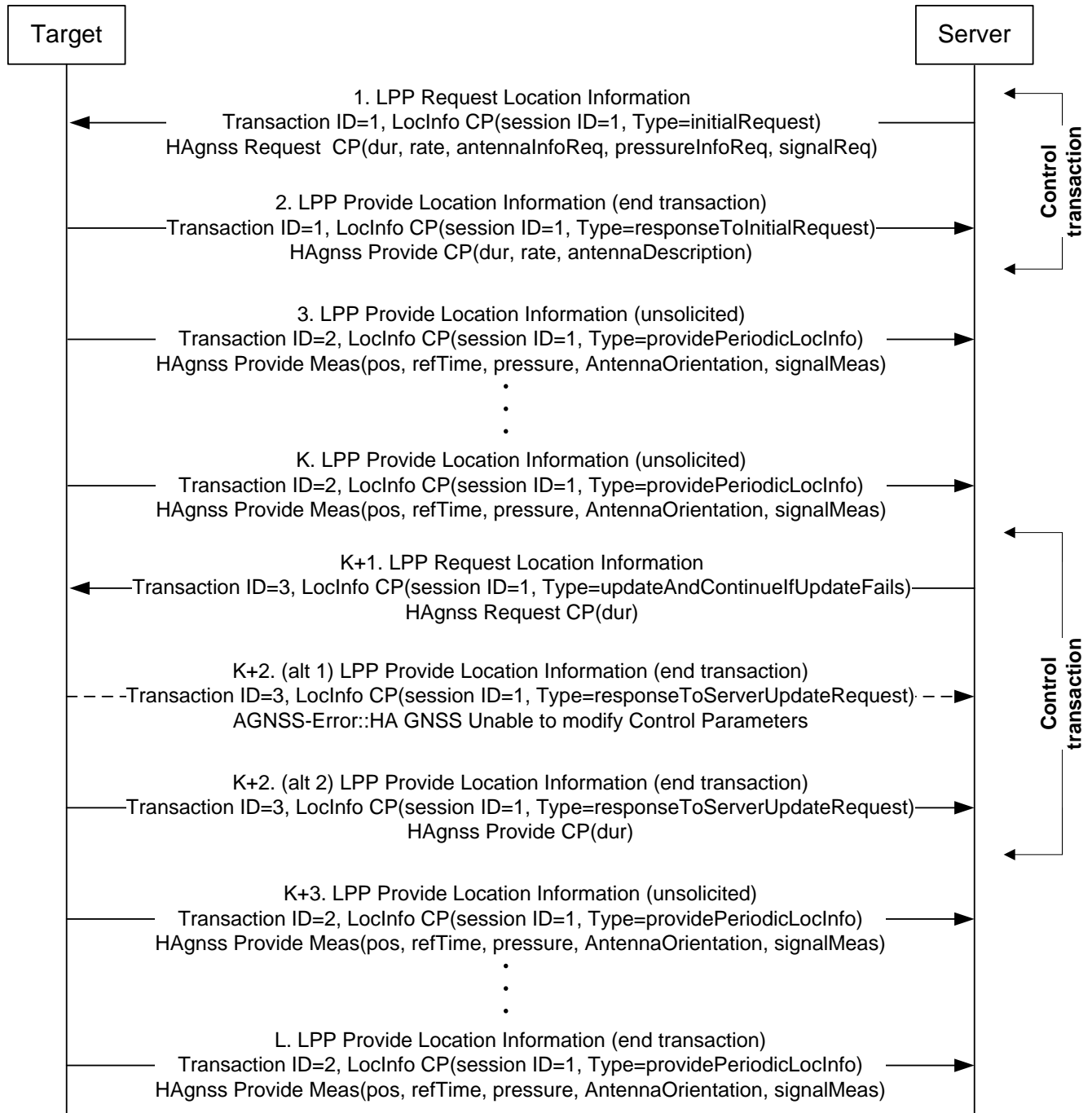
Figure 28: Periodic HA GNSS – nominal case
