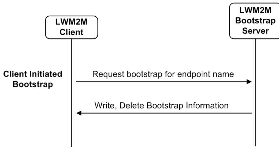
Figure 7: Procedure of Client Initiated Bootstrap
