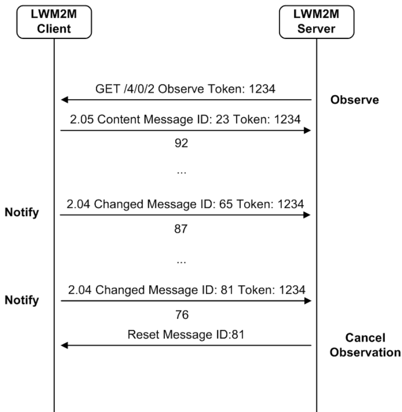
Figure 22: Example of an Information Reporting exchange.
