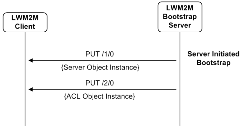
Figure 18: Example of Server initiated Bootstrap exchange.
