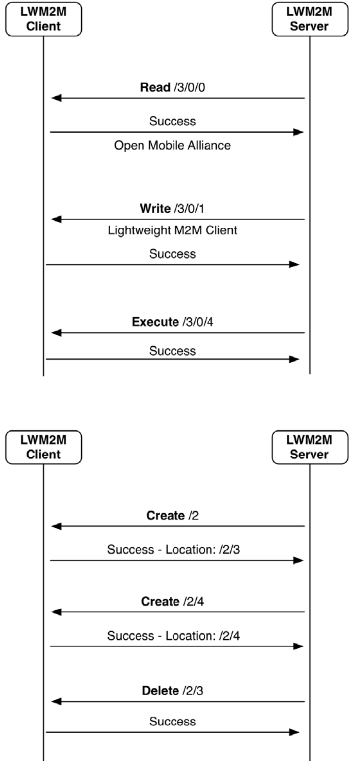
Figure 10: Example flows of Device Management & Service Enablement Interface
