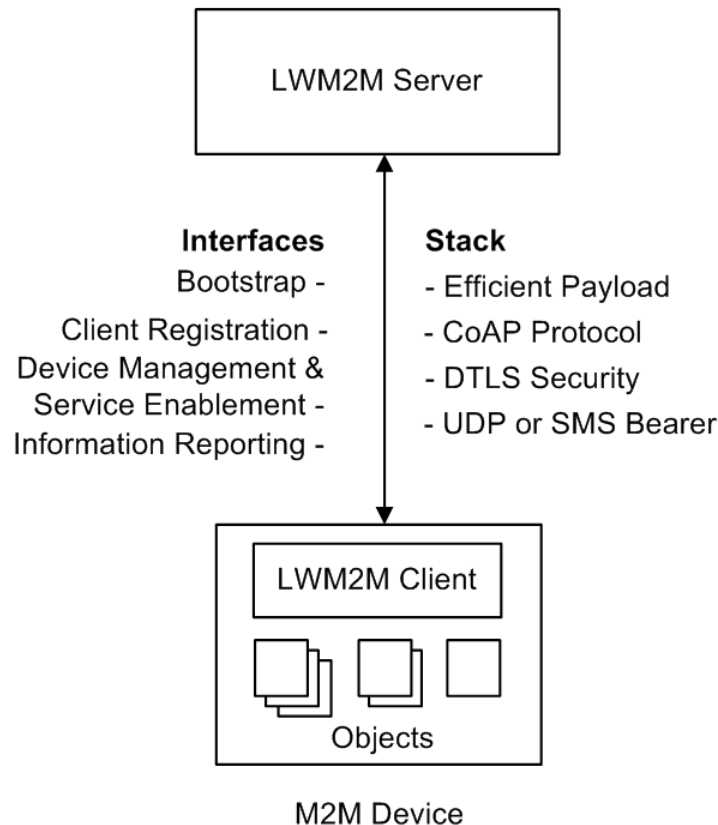
Figure 1: The overall architecture of the LWM2M Enabler.
