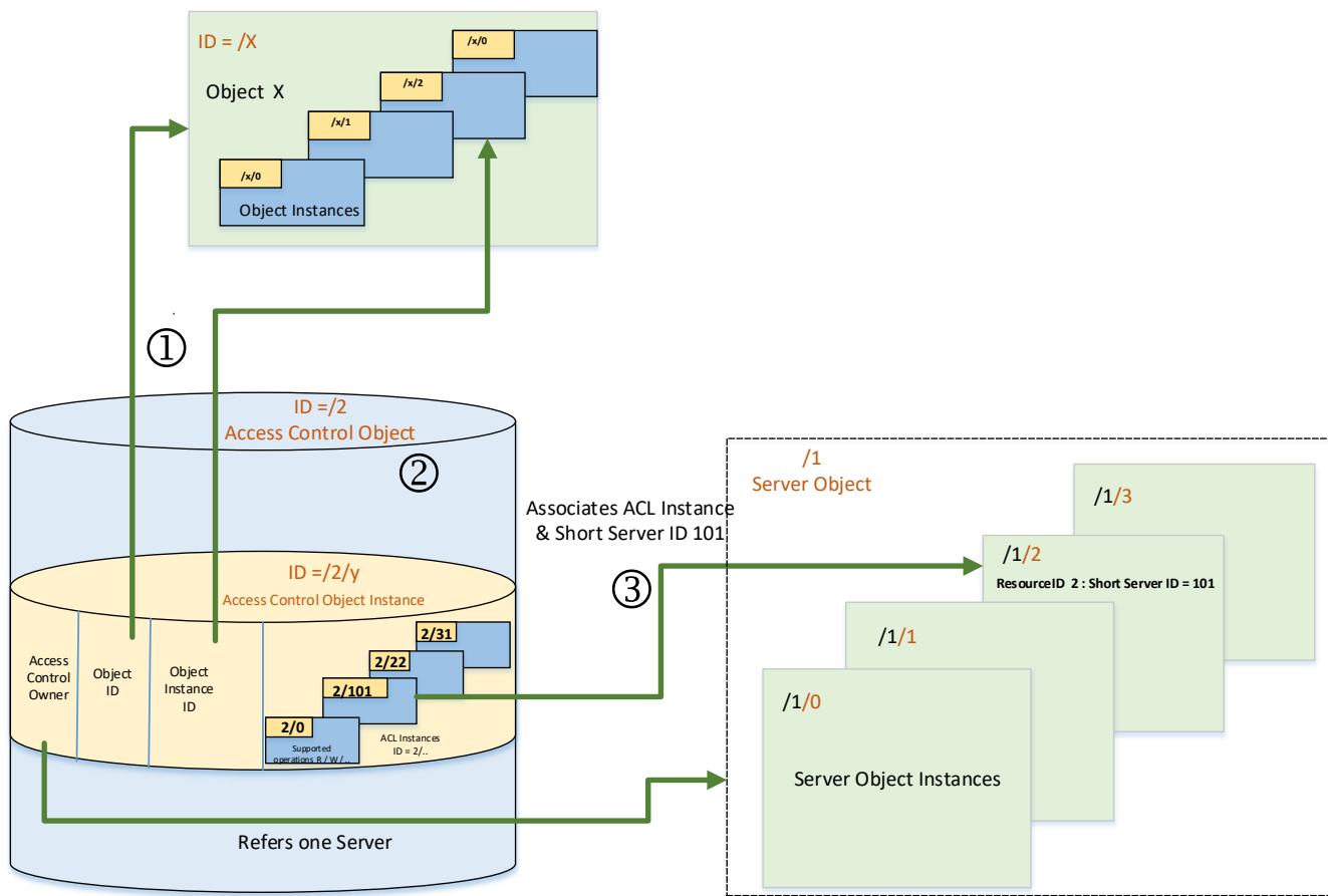
Figure 18: Illustration of the relations between the LwM2M Access Control Object and the other LwM2M Objects
