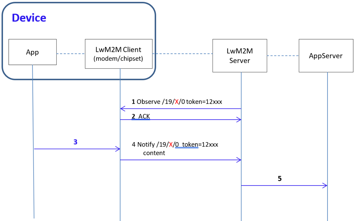
Figure: 5.2.-1 LwM2M Client Reports Application Data
