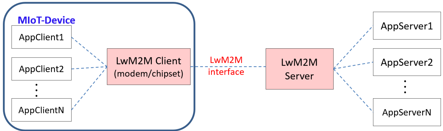
Figure: 5.1.-1 Application data transfer by LwM2M architecture
