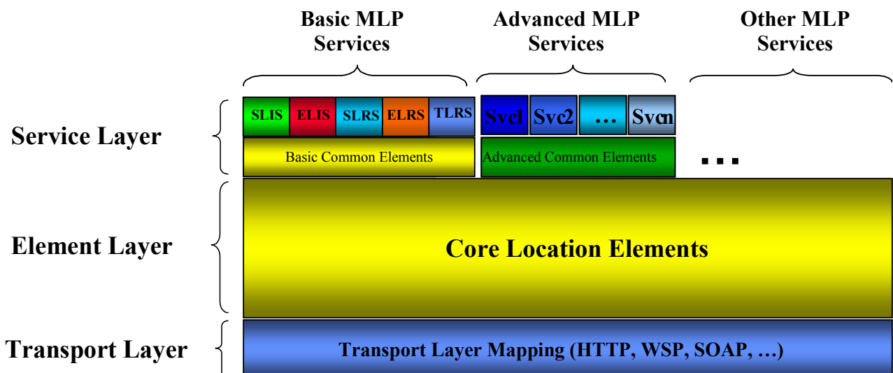
Figure 2: MLP Structure
