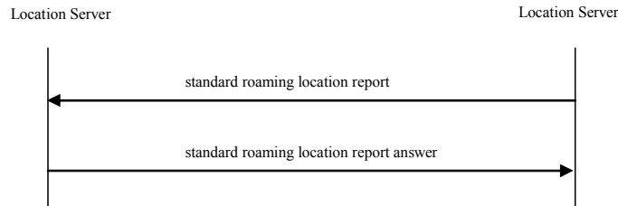
Figure 6: Standard Roaming Location Report
