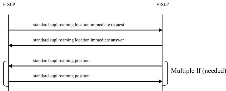
Figure 5: Standard SUPL Roaming Location Immediate
