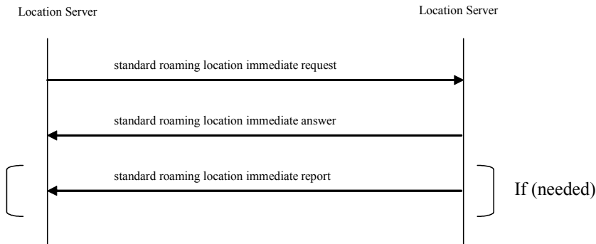
Figure 2: Standard Roaming Location Immediate
