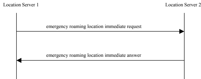
Figure 4: Emergency Roaming Location Immediate
