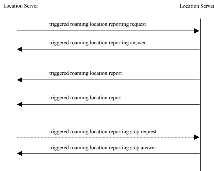
Figure 3: Triggered Roaming Location Reporting
