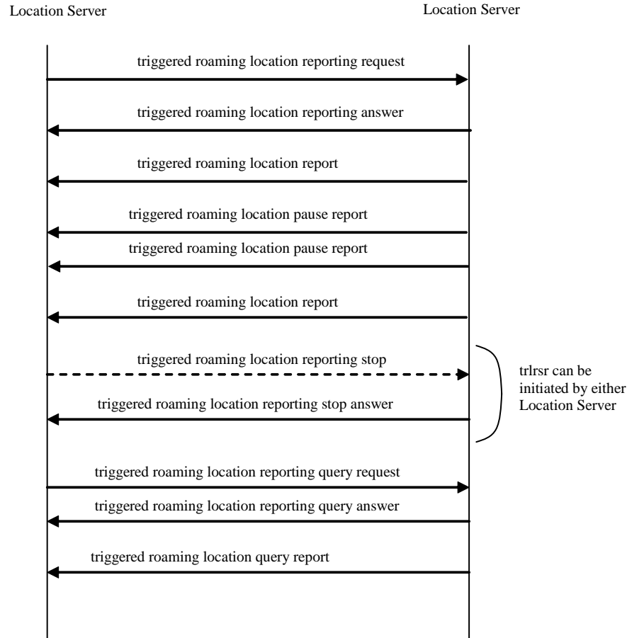
Figure 3: Triggered Roaming Location Reporting
