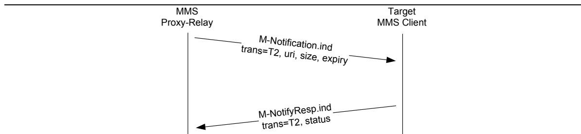
Figure 10. Example MMS Notification Transaction
