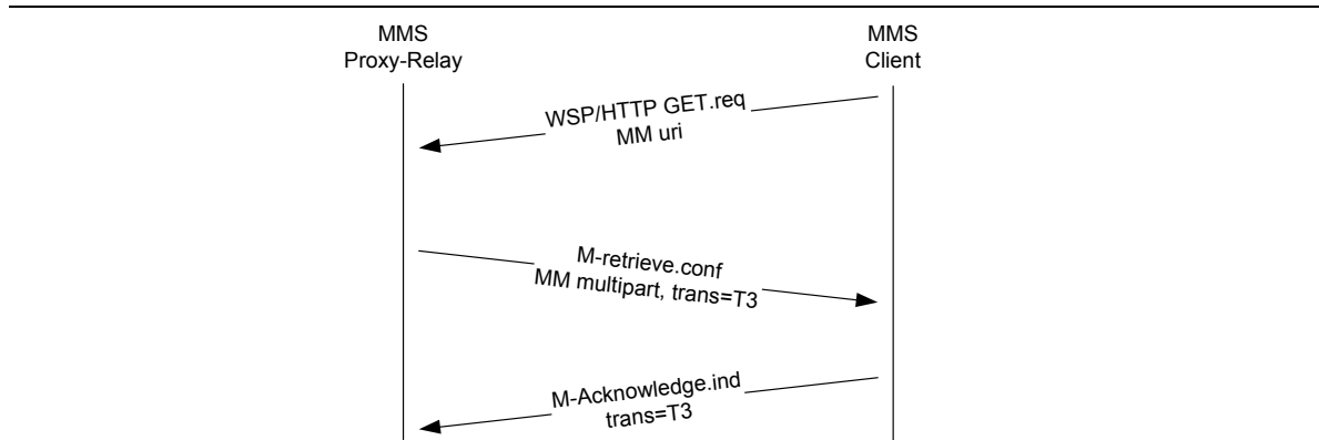
Figure 12. Example MMS Retrieval Transaction with Acknowledgement
