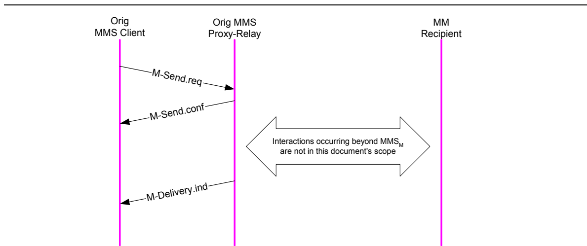
Figure 4. Example MMS_M Transaction Flow – Sending
