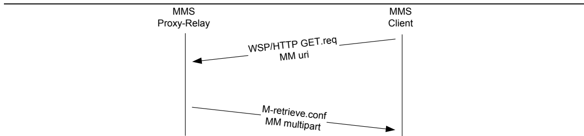
Figure 11. Example MMS Retrieval Transaction without Acknowledgement
