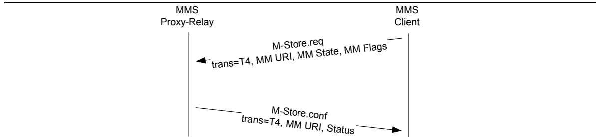
Figure 17. Example MMS Mbox-StoreTransaction
