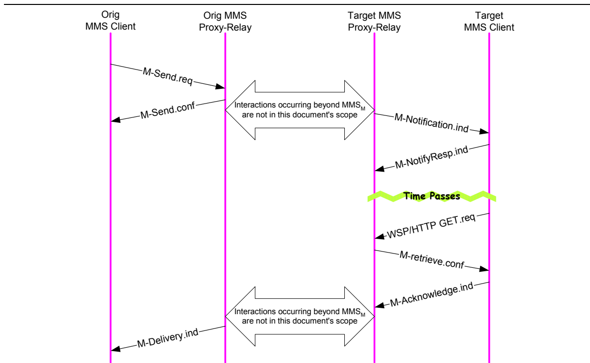
Figure 7. Example MMS Transaction Flow – Deferred Retrieval
